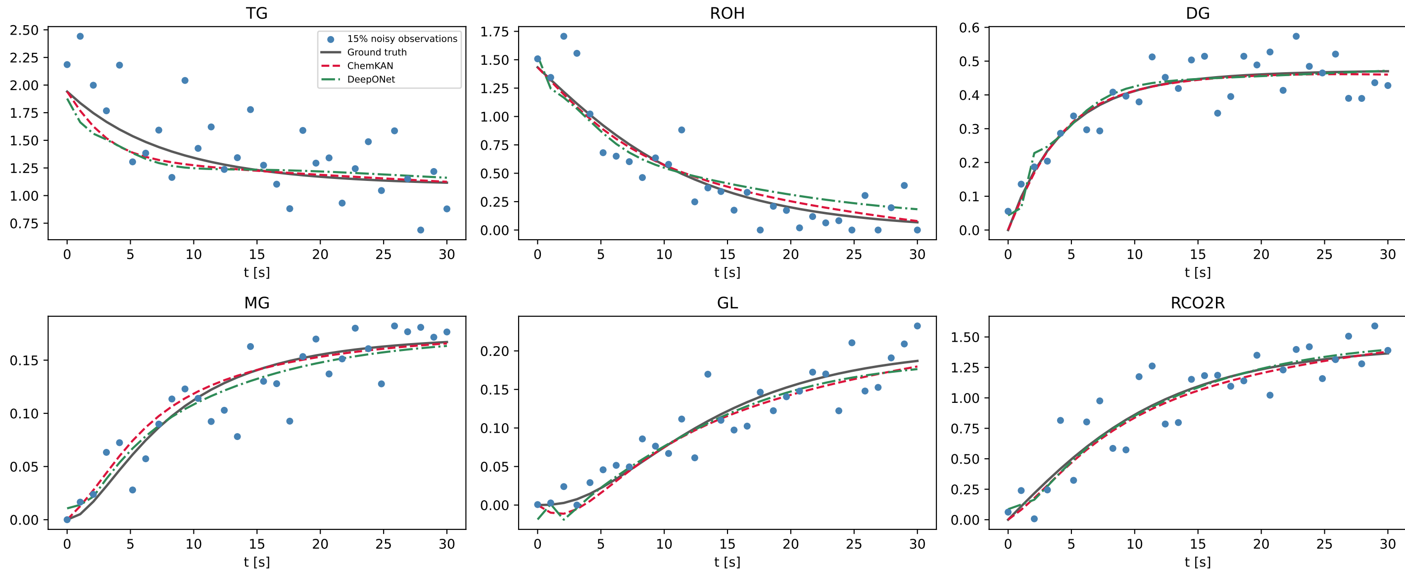
Fig. 6 - 15% noise, test row 24 (TG0=1.941, ROH0=1.433, T=334.75 K), biodiesel_v2 runs noise-free time-averaged MSE (Eq. 18 / 30): ChemKAN 3.44e-04, DeepONet (tanh, lr 1e-2) 7.32e-04 ChemKAN evaluated at rtol 1e-06, atol 1e-10 (training: rtol 1e-2, atol 1e-6)
