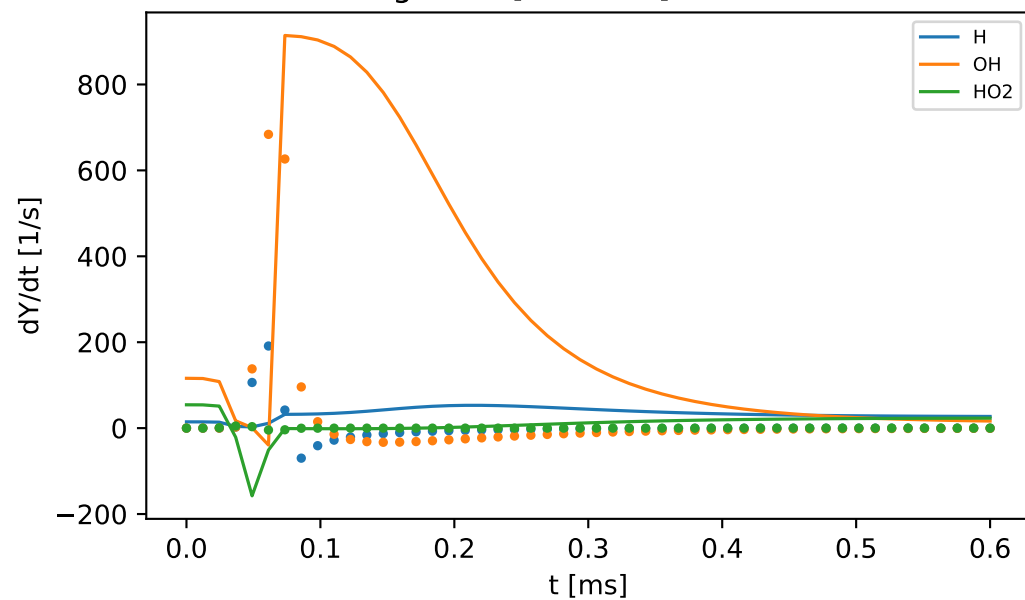
B. dY/dt along truth [held-out] relative L2 = 2.25
