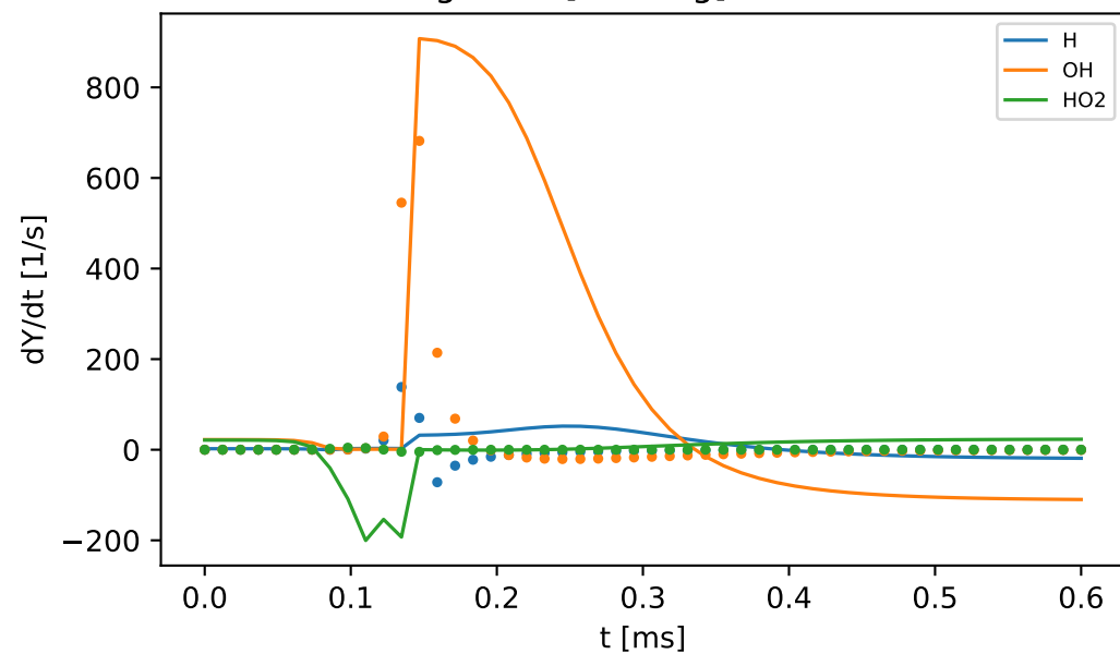
B. dY/dt along truth [training] relative L2 = 2.03
