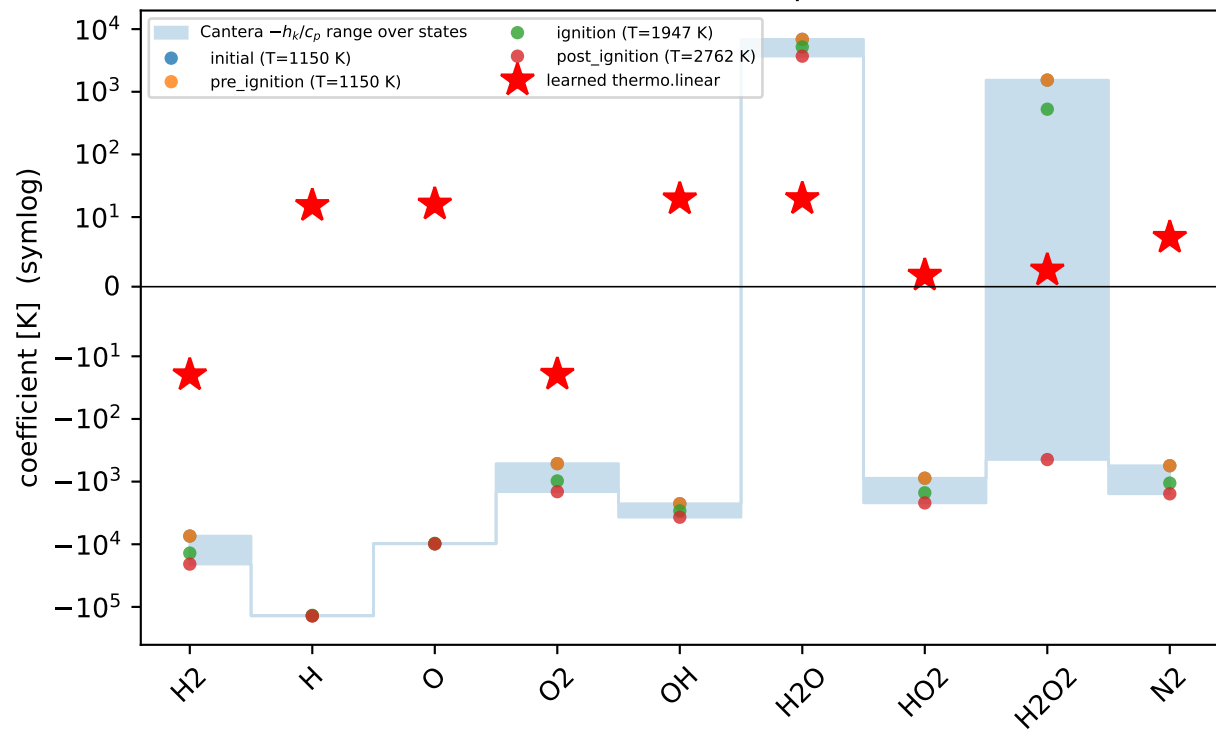
held-out T0=1150 K, phi=1.3
