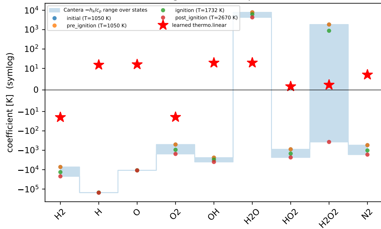
training T0=1050 K, phi=0.9
