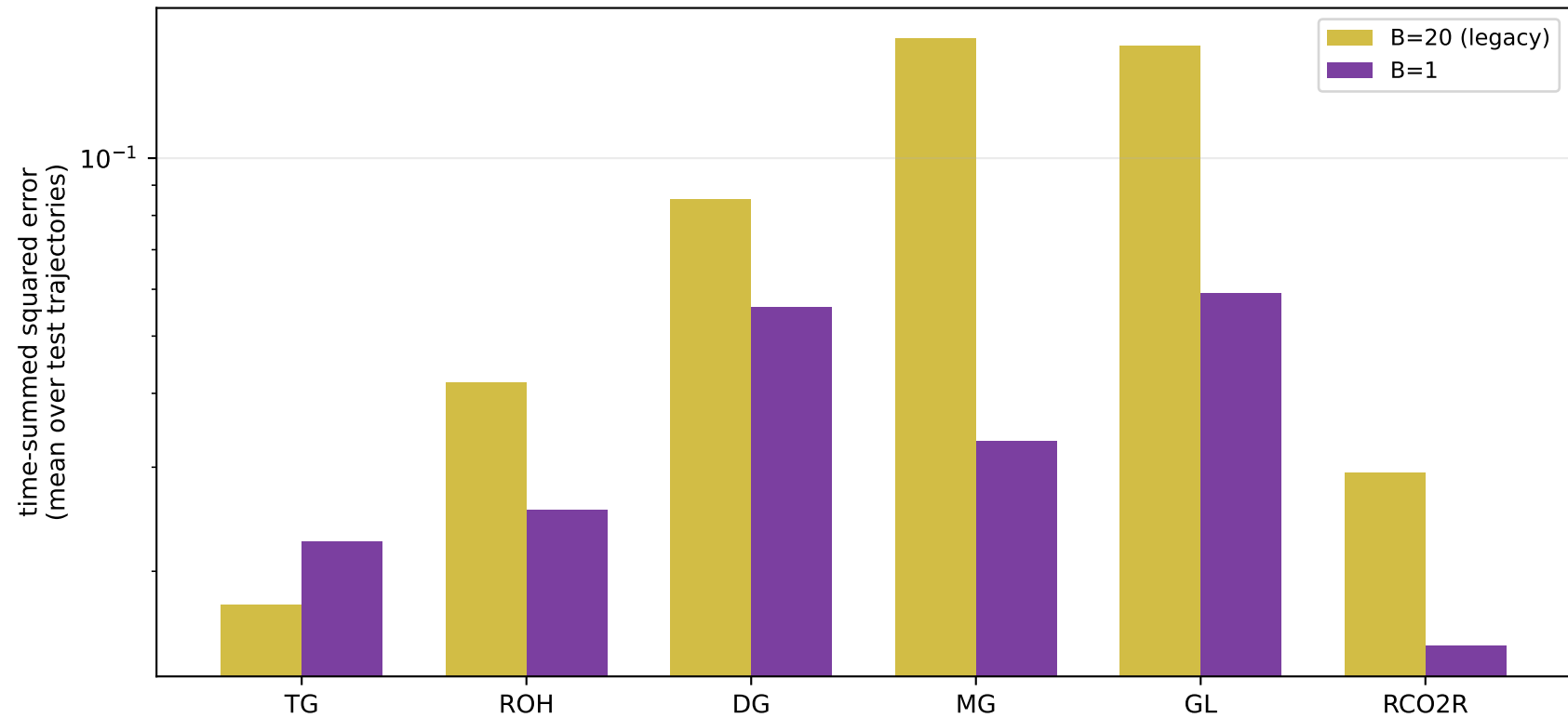
Held-out error by species (10 test conditions)
