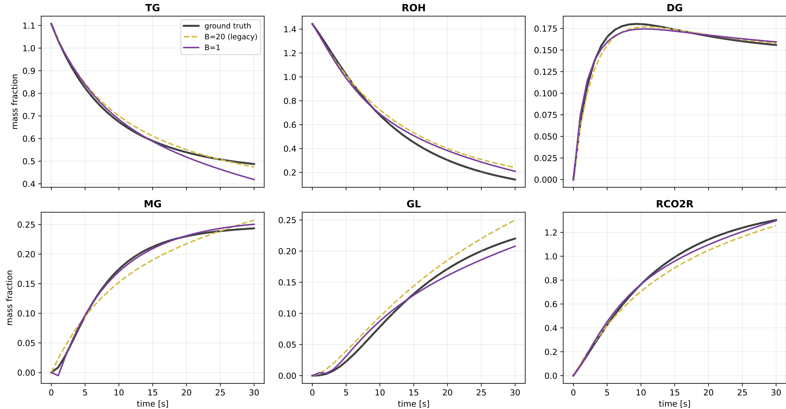
Held-out test case 0 ( T = 338.2 K) — prediction from u(0) only
