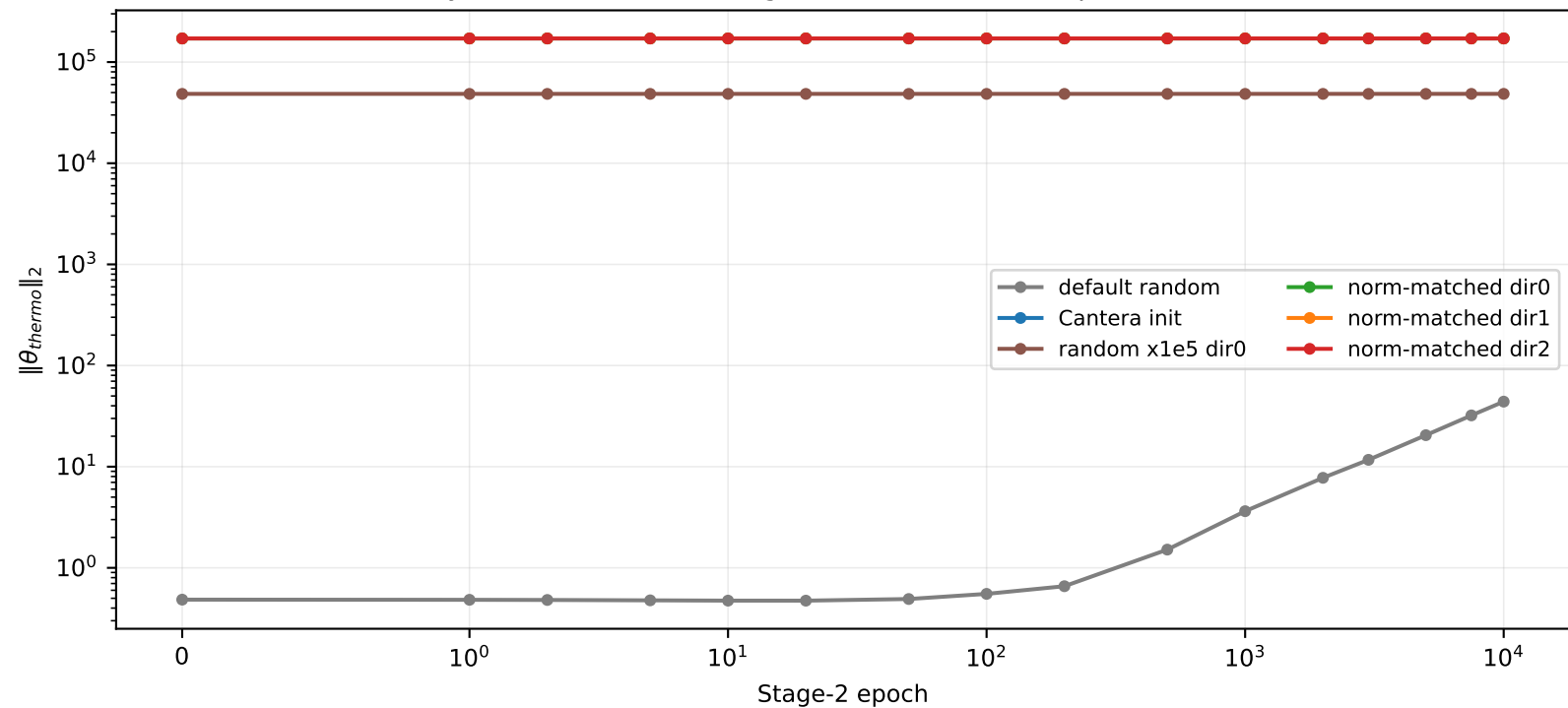
Thermodynamic coefficient magnitude over 10 000 epochs [DIAGNOSTIC]
