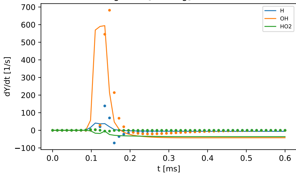
B. dY/dt along truth [training] relative L2 = 1.52
