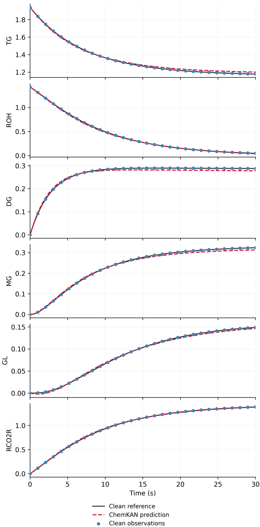
Figure 3 | 0% training noise Observed-interval training, seed 0; 10,000 updates TG = 1.94, ROH = 1.43; other species = 0 T = 334.8 K | Complete rollout
