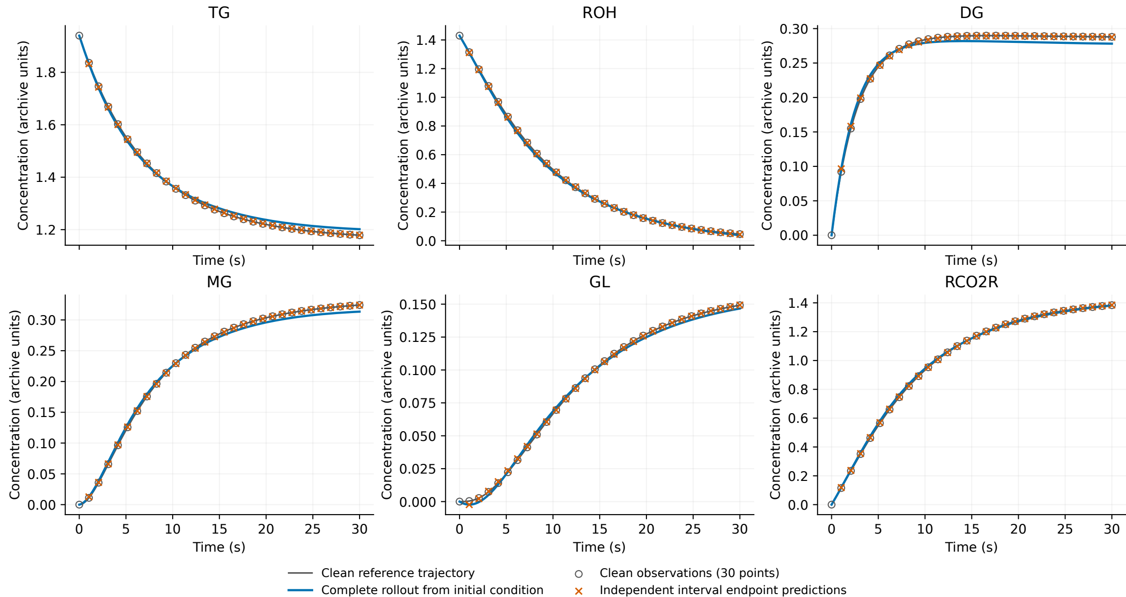
Figure 3 endpoint diagnostic | Clean interval-trained model, seed 0 TG = 1.94, ROH = 1.43, DG = MG = GL = RCO2R = 0; T = 334.8 K Orange endpoints use fresh observed states; the blue rollout uses only the initial condition
