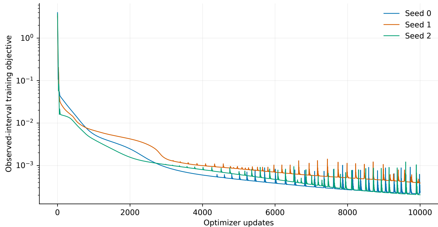
Observed-interval objective convergence Sum over 29 endpoints; mean over 6 species and 20 training conditions
