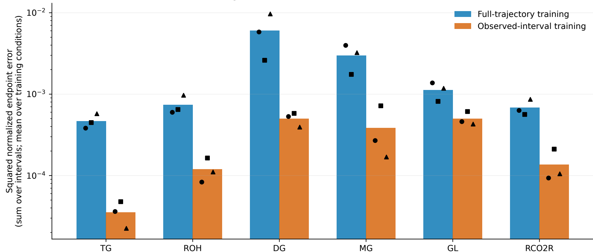
Interval error by species at 10,000 updates Both training methods evaluated with observed-state resets
