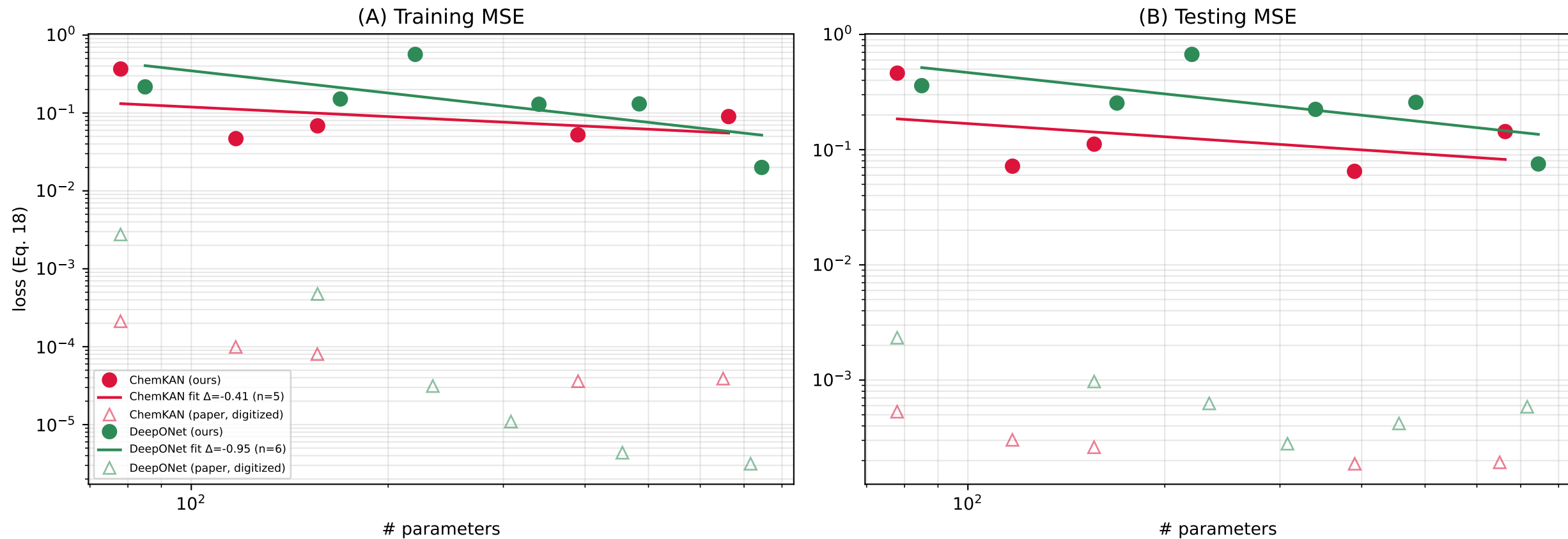
Fig. 4 - neural scaling. Filled = our runs; open = the paper's own digitized points (different absolute scale; shown for shape, not agreement)
