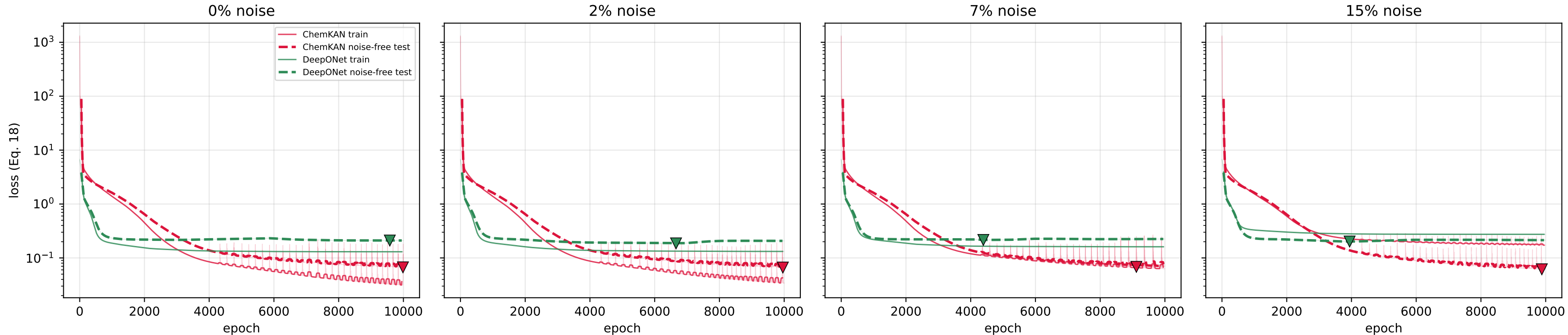
Fig. 5B - faint = RAW per-epoch values; bold = display-only 101-epoch moving average; markers = clean-test minima of the RAW curves
