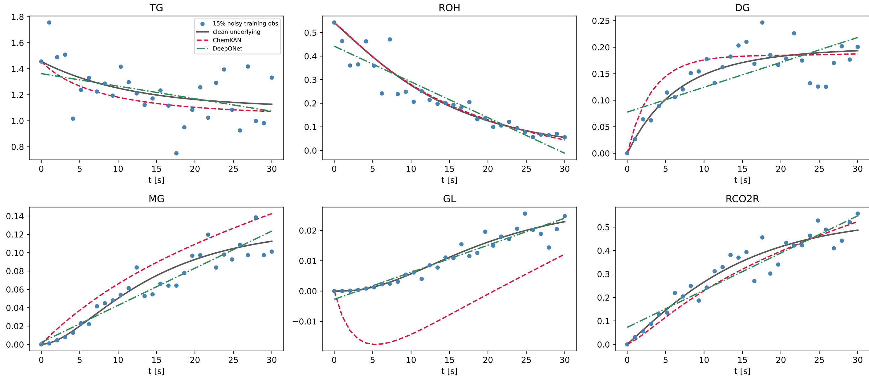
Fig. 6 - 15% noise, training case 0 (TG0=1.4554, ROH0=0.5425, T=334.43 K) - plotting choice
