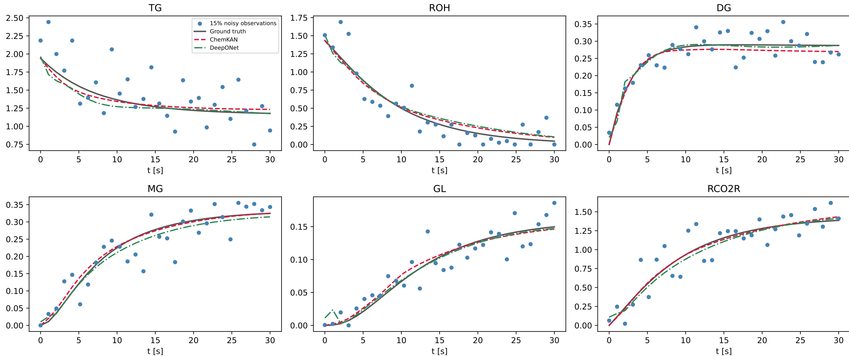
Fig. 6 - 15% noise, test row 24 (TG0=1.941, ROH0=1.433, T=334.75 K), PAPER reaction order noise-free time-averaged MSE (Eq. 18 / 30): ChemKAN 3.51e-04, DeepONet (tanh, lr 1e-2) 5.41e-04
