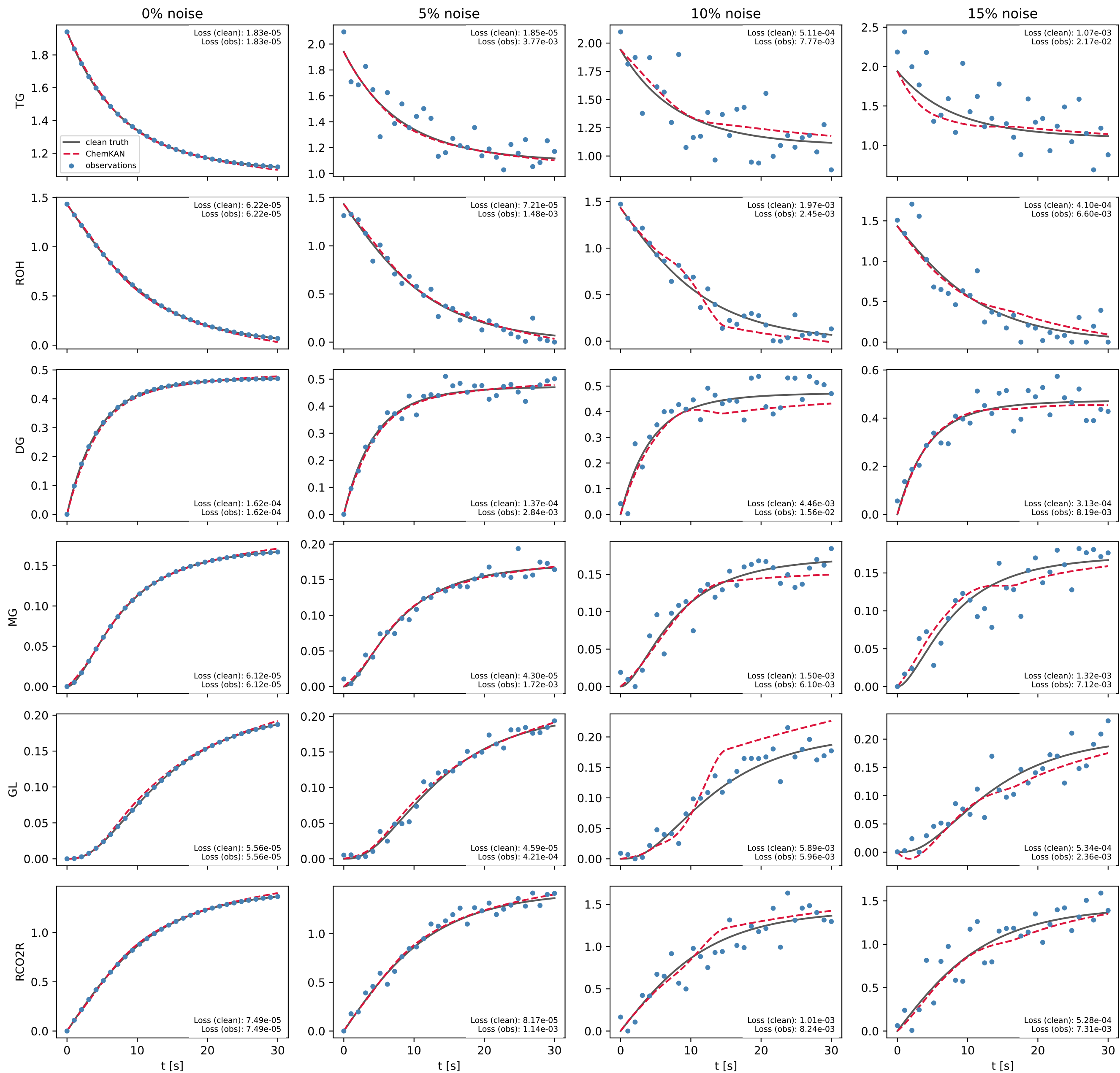
Fig. 3 - TG0=1.941, ROH0=1.433, T=334.75 K (paper-explicit unseen condition) biodiesel_v2 runs (test row 24); loss: time-averaged MSE (Eq. 18 / 30)
