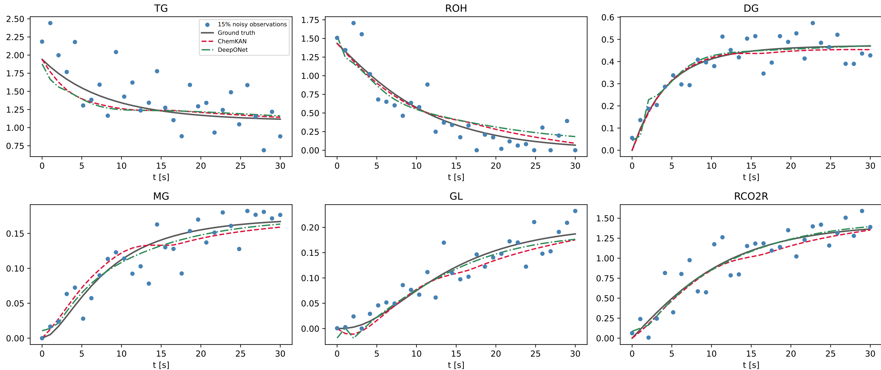
Fig. 6 - 15% noise, test row 24 (TG0=1.941, ROH0=1.433, T=334.75 K), biodiesel_v2 runs noise-free time-averaged MSE (Eq. 18 / 30): ChemKAN 6.95e-04, DeepONet (tanh, lr 1e-2) 7.32e-04
