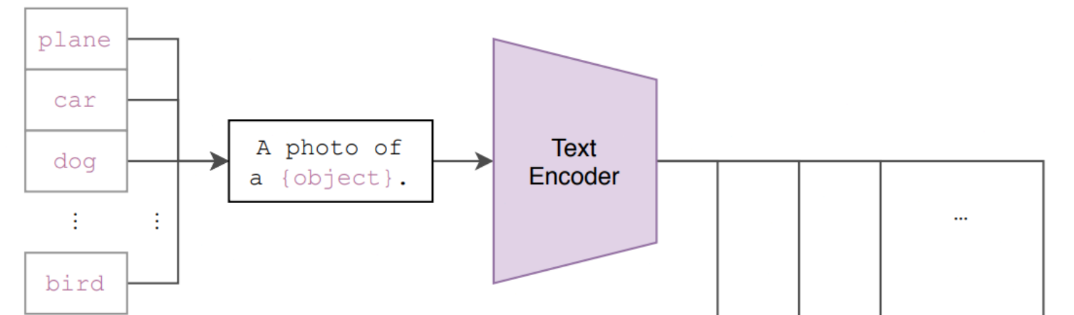
(2) Create dataset classifier from label text
