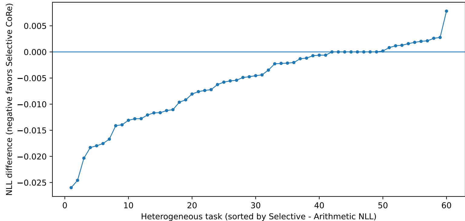
Selective CoRe adapts across heterogeneous reliability tasks
