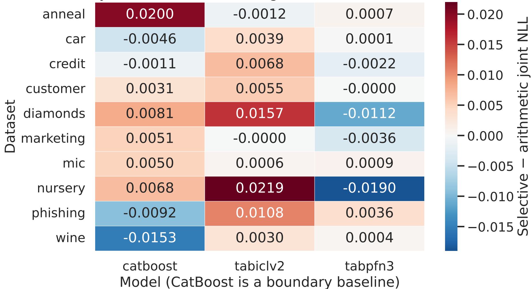
Effect by dataset and model (negative favors Selective CoRe)
