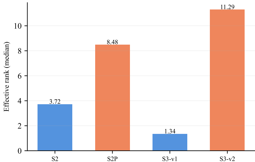
(b) Effective rank of decoder Jacobian
