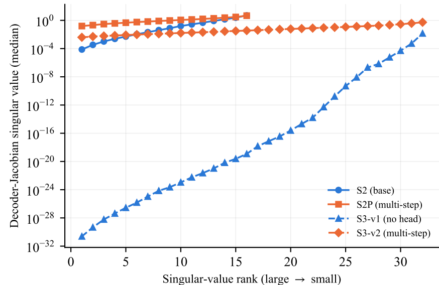
(a) Jacobian singular-value spectra
