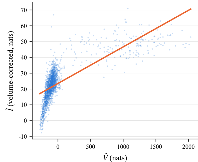
(a) \hat{I} - \hat{V} (s5): R^2 = 0.54 , \rho = 0.41
