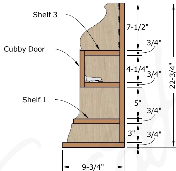
Side Section
