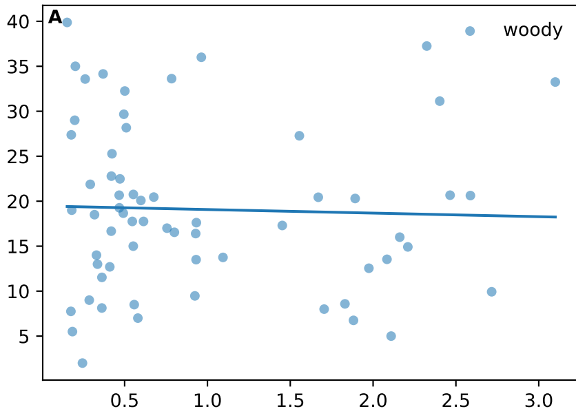
EcoBank_prop_rhizophilic_mean vs root_diameter_mean
