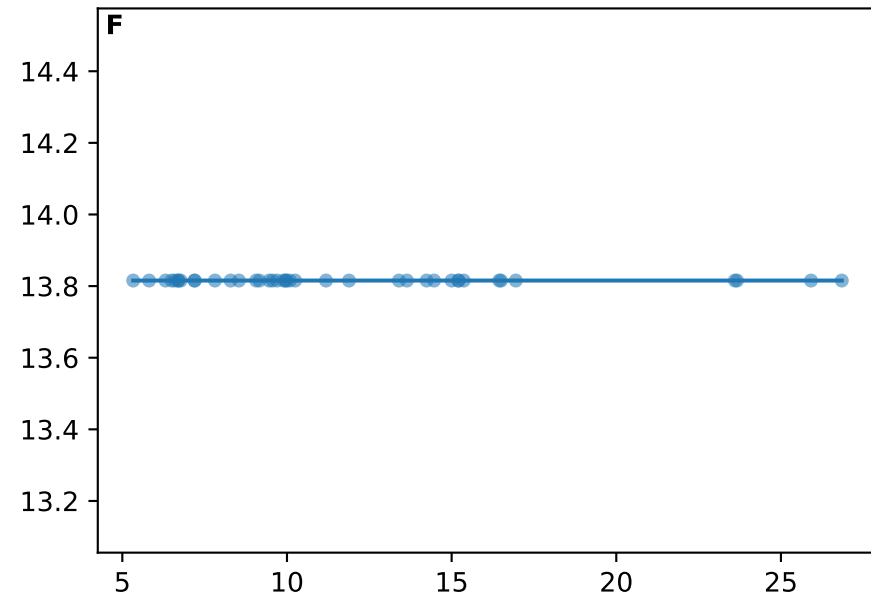
EcoBank_prop_rhizophilic_mean vs root_N_mean
