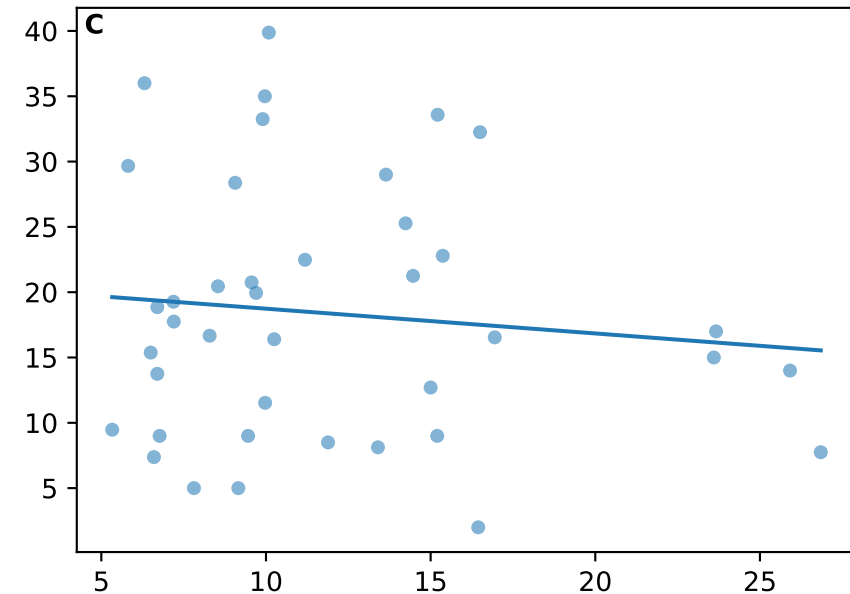
EcoBank_prop_rhizophilic_mean vs root_N_mean
