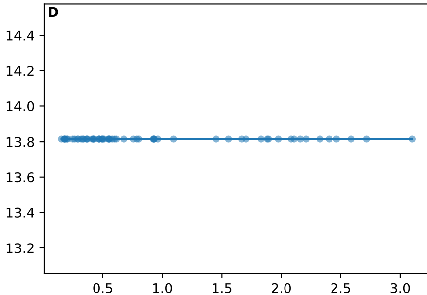
EcoBank_prop_rhizophilic_mean vs root_diameter_mean
