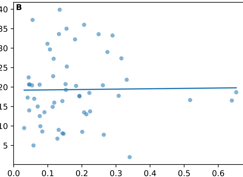
EcoBank_prop_rhizophilic_mean vs RTD_mean
