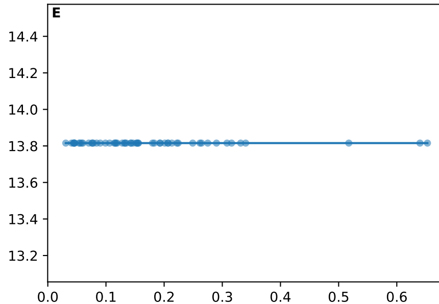
EcoBank_prop_rhizophilic_mean vs RTD_mean
