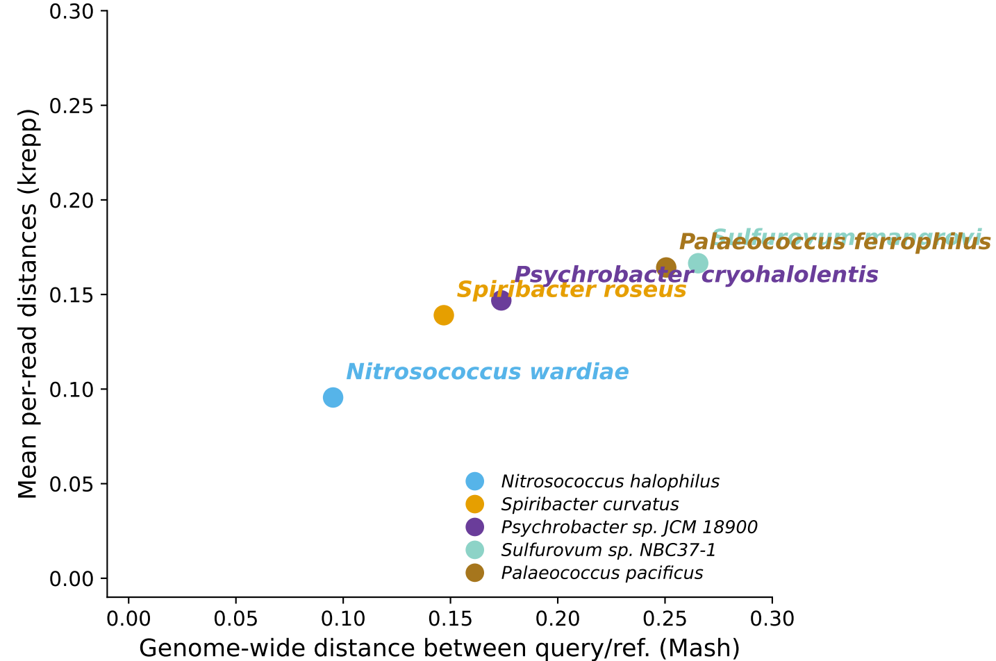
Genus-level queries
