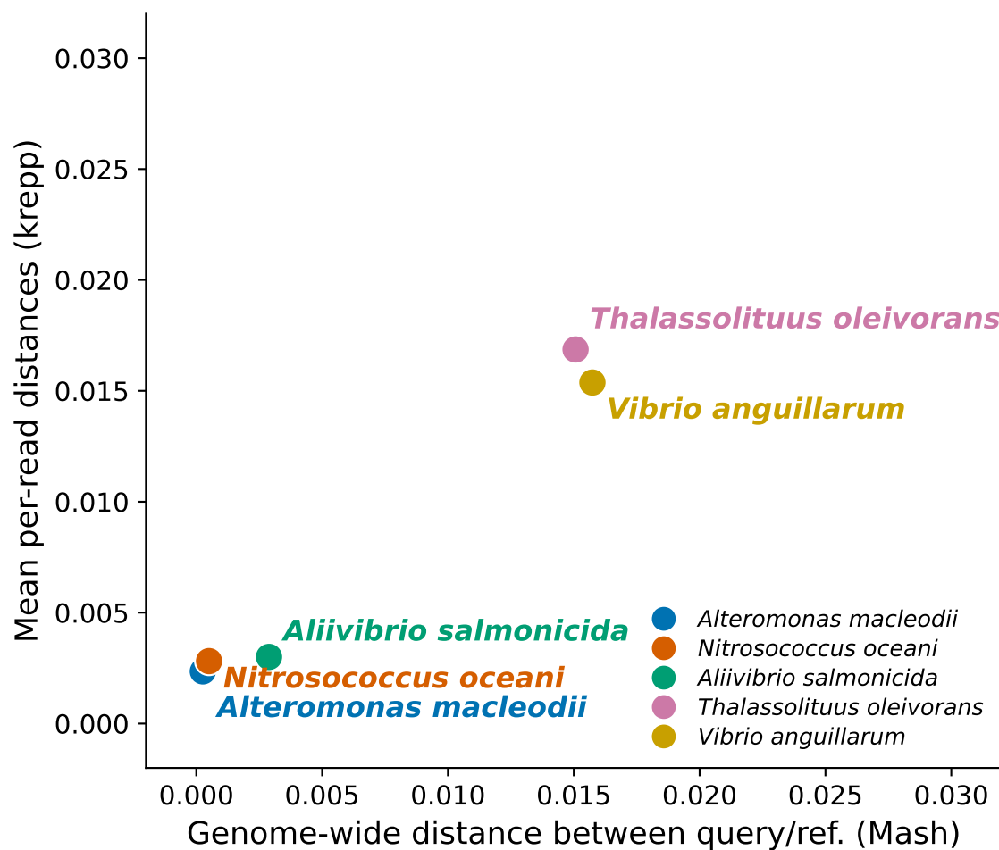
Species-level queries
