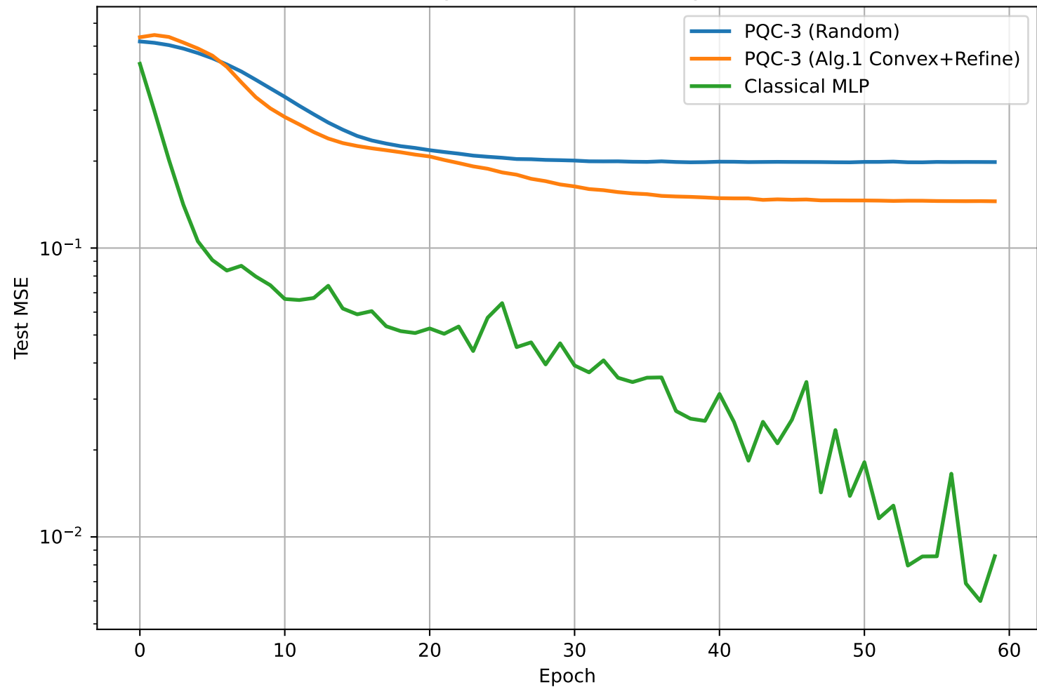
Learning Curves (Test MSE, log-scale)
