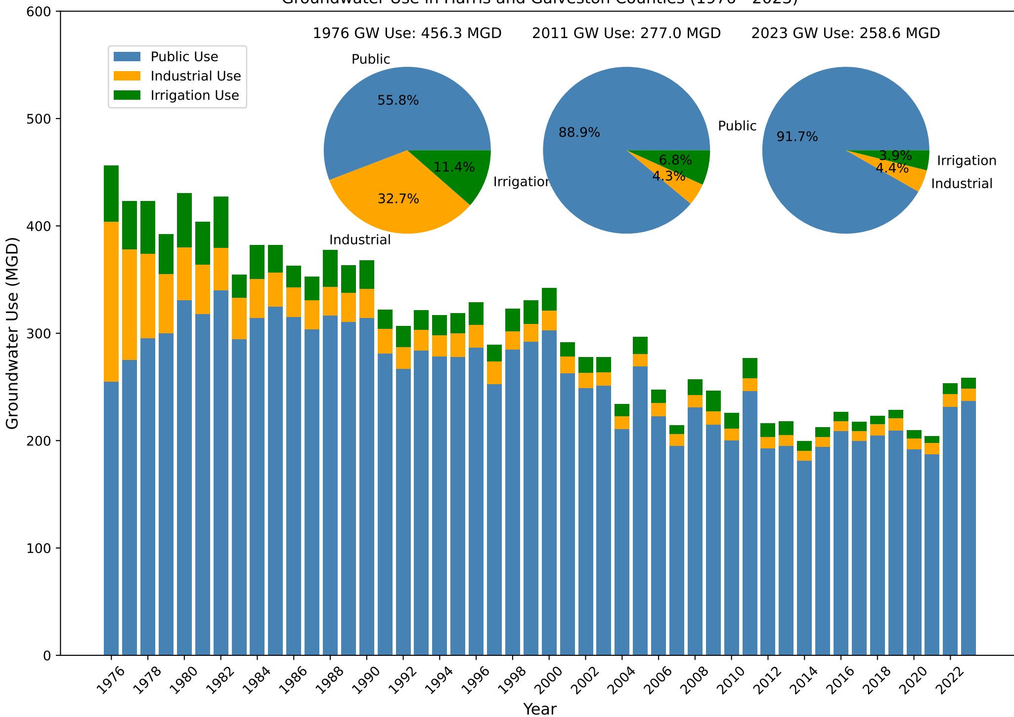
Groundwater Use in Harris and Galveston Counties (1976 - 2023)
