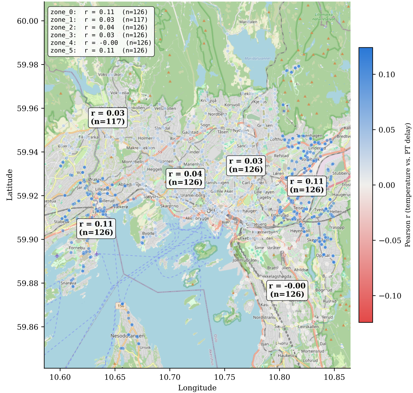
(b) Spatial variation: temperature vs. PT delay — W-C (2026-03-07 - 2026-03-14)
