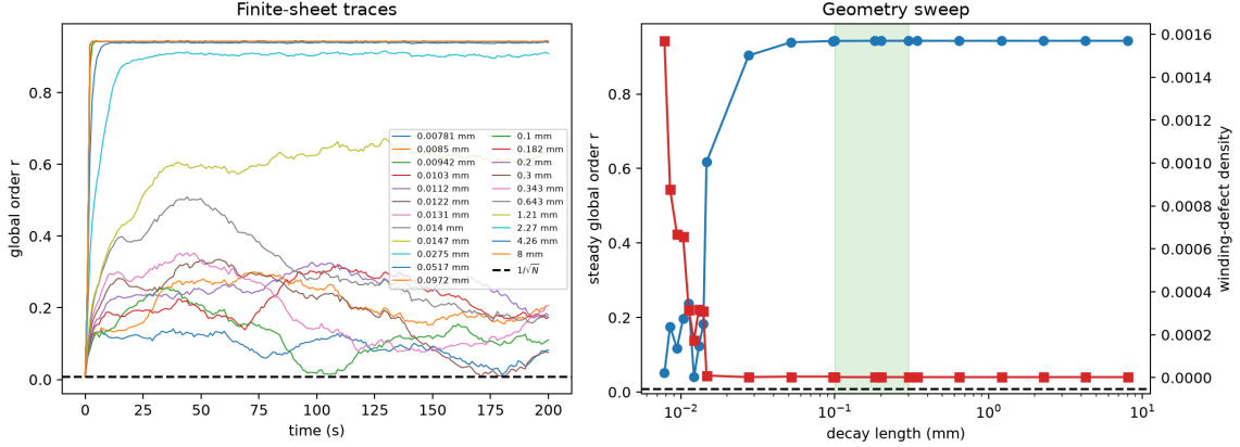
Figure 1: Finite-sheet heuristic evidence under a row-normalised spatial kernel. The left panel shows global order traces and the 1/\sqrt{N} finite-size floor; the right compares steady order and wrapped plaquette winding-defect density across physical decay lengths. The shaded band is 0.1–0.3 mm. This sampled simulation establishes no general transition or biological identification.
