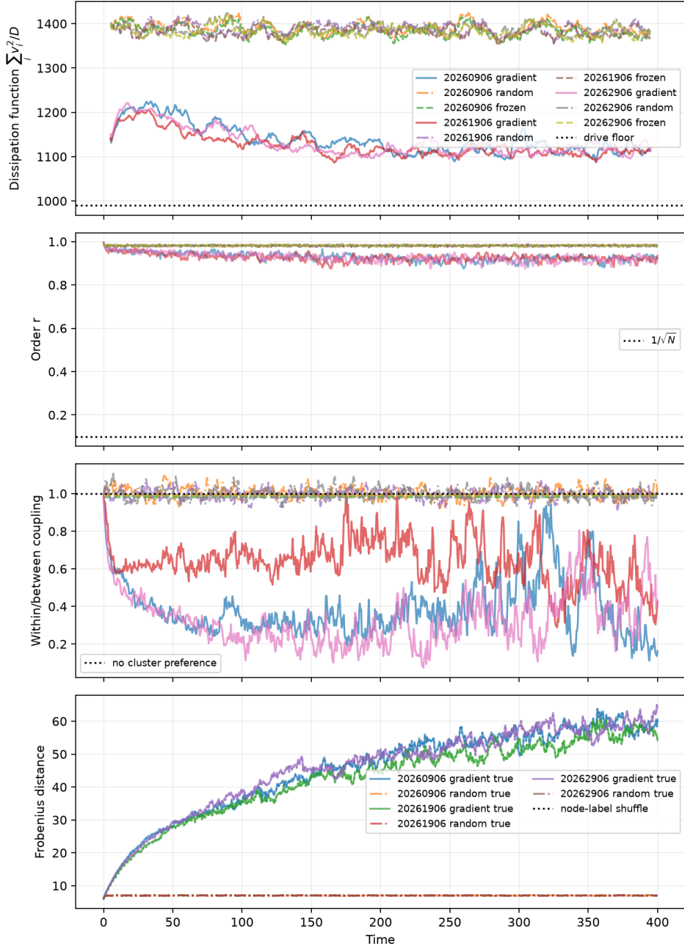
Figure S3: Joint fast/slow dynamics in three finite seeded runs, three arms each: gradient (solid), matched-norm random step (dash-dotted), frozen kernel (dashed). First: dissipation function, smoothed over 21 saved samples, against the N\langle\omega\rangle^2/D floor the conserved mean drift imposes. Second: order and the 1/\sqrt{N} reference. Third: mean within-cluster over mean between-cluster coupling, with the no-preference line at unity. Fourth: distances to the cluster template (solid) and its node-label shuffle (dotted), which grow together as the kernel norm grows. Only the gradient arm descends the objective, and only it loses cluster alignment; these diagnostics provide no evidence of structural resonance or a thermodynamic entropy-production rate.
