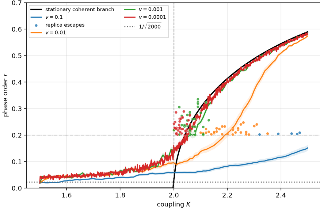
Figure S3: Finite-rate departures from the stationary branch. Curves show ensemble-mean order for four ramp speeds v , with one-standard-error bands. Coloured points mark each replica's first sustained escape, plotted at its recorded order; censored replicas have no point. The dashed vertical line is the static threshold, the dash-dotted horizontal line is the escape criterion, and the dotted horizontal line is the finite-size reference. The replica-bootstrap interval for the delay exponent is reported below.
