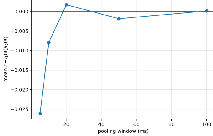
Figure 4: Sensitivity of the mean collapse residual to the spatiotemporal pooling window. This assesses the pooled estimator and does not turn 62-channel EEG into an instantaneous spatial sample.
