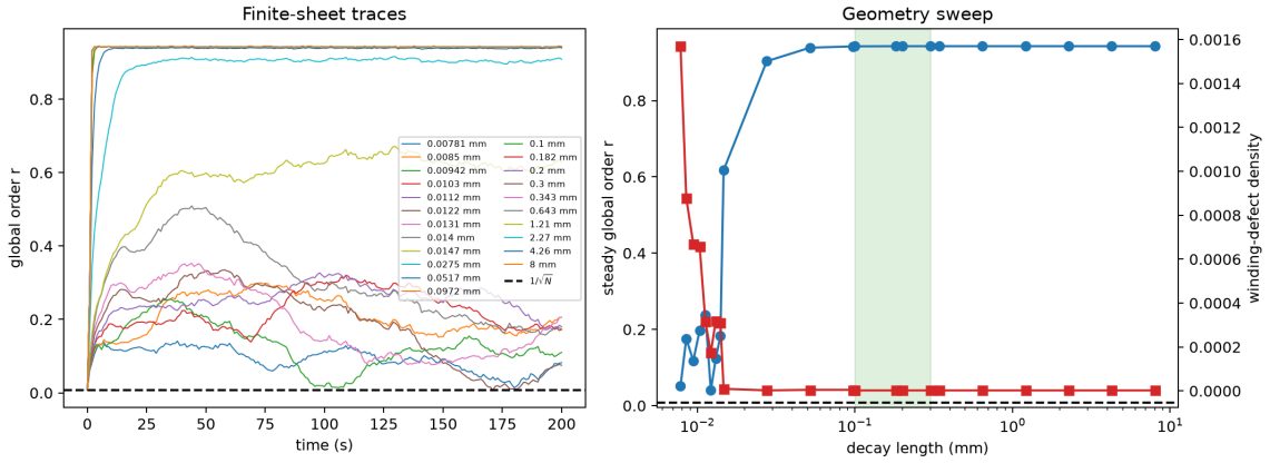
Figure 3: Finite-sheet heuristic evidence under a row-normalised spatial kernel. The left panel shows global order traces and the 1/\sqrt{N} finite-size floor; the right compares steady order and wrapped plaquette winding-defect density across physical decay lengths. The shaded band is 0.1–0.3 mm. This sampled simulation establishes no general transition or biological identification.
