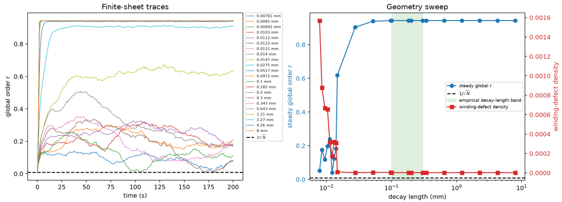
Figure S4: Finite-sheet heuristic evidence under a row-normalized spatial kernel. The left panel shows global order traces and the 1/\sqrt{N} finite-size floor; the right compares steady order and wrapped plaquette winding-defect density across physical decay lengths. The shaded band is 0.1–0.3 mm. This sampled simulation establishes no general transition or biological identification.
