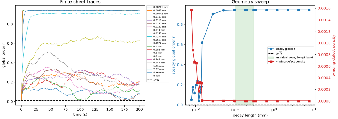
Figure S4: Finite-sheet heuristic evidence under a row-normalized spatial kernel. The left panel shows global order traces and the 1/\sqrt{N} finite-size floor; the right compares steady order and wrapped plaquette winding-defect density across physical decay lengths. The shaded band is 0.1–0.3 mm. This sampled simulation establishes no general transition or biological identification.
