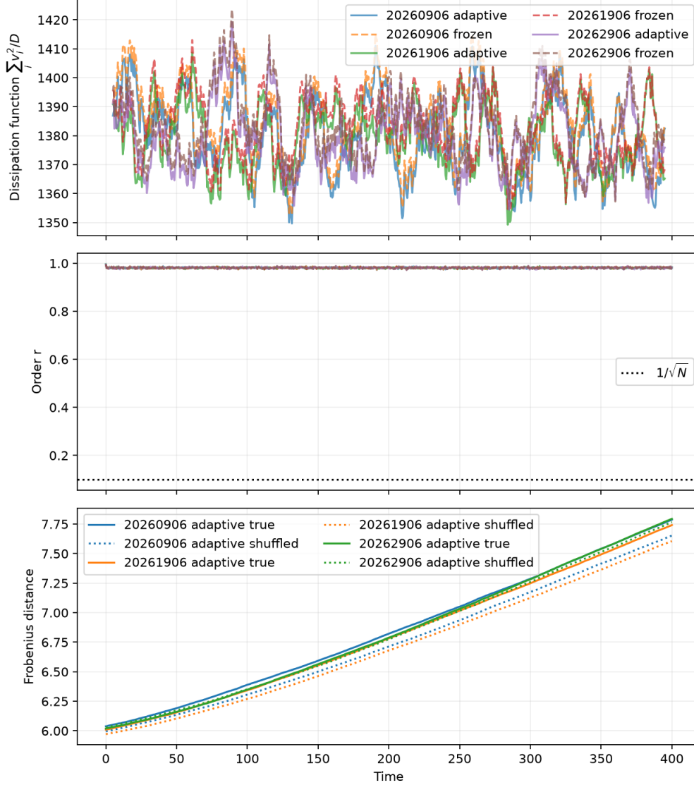
Figure S3: Joint fast/slow dynamics in three finite seeded runs. Top: dissipation function, smoothed over 21 saved samples, with matched frozen-coupling controls (dashed). Middle: order and the 1/\sqrt{N} reference. Bottom: distances to the cluster template (solid) and its node-label shuffle (dotted). Coherence persists, but template distances increase; these diagnostics provide no evidence of structural resonance or a thermodynamic entropy-production rate.
