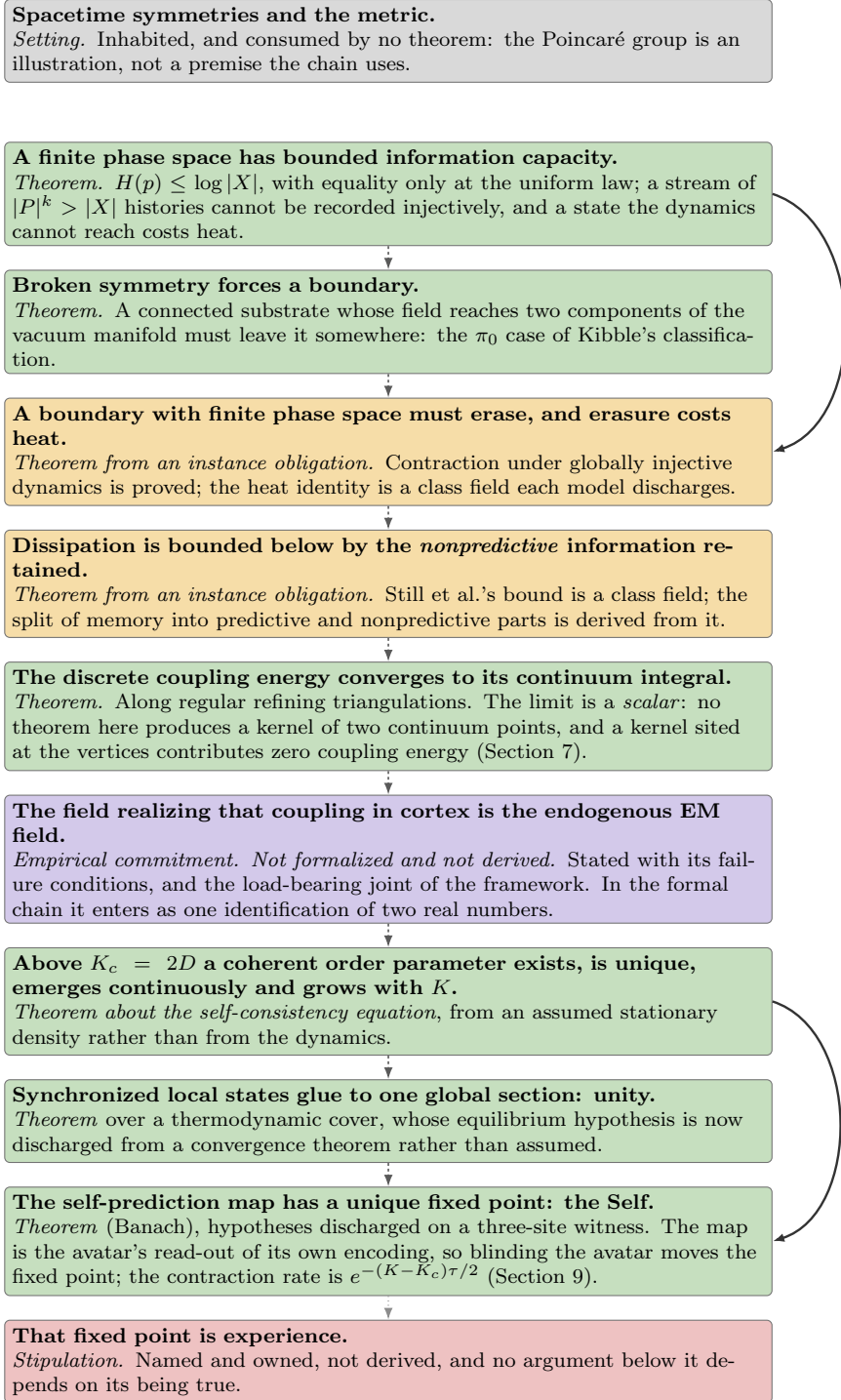
Figure 1: The conditional composition schema, with eight assumed vertical arrows and the status of each node and of each arrow. Nodes. ■ theorem; ■ theorem resting on a class field that each model must discharge; ■ empirical commitment, neither formalized nor derived; ■ stipulation; ■ setting, consumed by no theorem. Arrows. A solid arrow is a Lean theorem. A dashed arrow is a named hypothesis of chain (Chain.lean): an implication between the two node statements which the development does not prove
