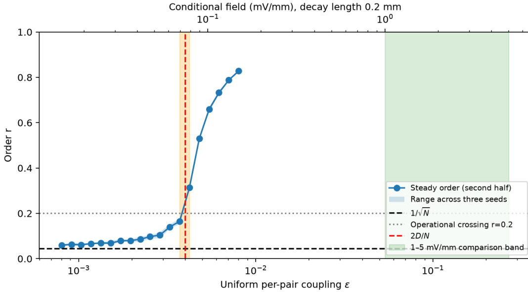
Figure 2: Finite- N rescue in the declared weak-synapse regime. Points are three-seed mean order; blue shading gives the seed range. Orange shading marks the union of sampled crossing brackets. The top axis uses the conditional \gamma = 1 field conversion at decay length 0.2 mm; green shading is the 1–5 mV/mm comparison band. The dashed horizontal line is 1/\sqrt{N} . The balanced strong-synapse control remains a distinct regime and does not satisfy the floor-level baseline gate.
