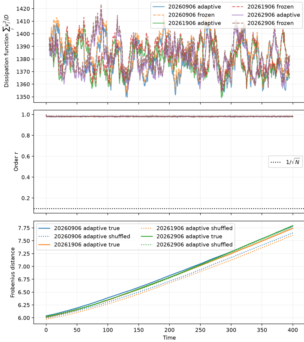
Figure 3: Joint fast/slow dynamics in three finite seeded runs. Top: dissipation function, smoothed over 21 saved samples, with matched frozen-coupling controls (dashed). Middle: order and the 1/\sqrt{N} reference. Bottom: distances to the cluster template (solid) and its node-label shuffle (dotted). Coherence persists, but template distances increase; these diagnostics provide no evidence of structural resonance or a thermodynamic entropy-production rate.
