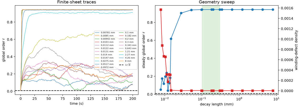
Figure 4: Finite-sheet heuristic evidence under a row-normalised spatial kernel. The left panel shows global order traces and the 1/\sqrt{N} finite-size floor; the right compares steady order and wrapped plaquette winding-defect density across physical decay lengths. The shaded band is 0.1–0.3 mm. This sampled simulation establishes no general transition or biological identification.
