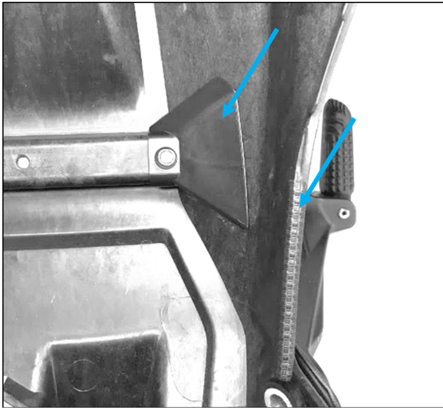
Fig. 9 - Install cable and edge protection inside
