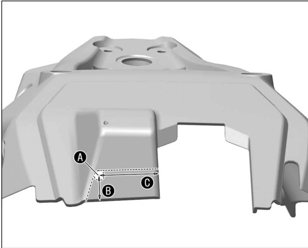
Fig. 7 - Position for holes on the lower rear part B = 15 mm C = 45 mm
