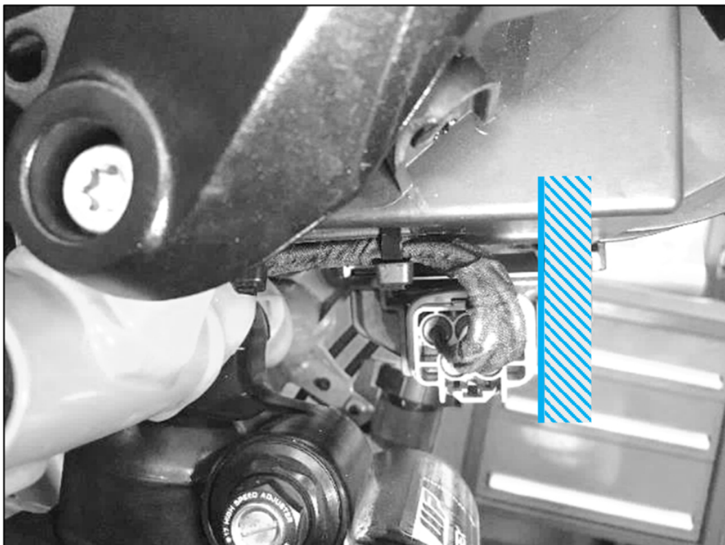
Figure 12 - Align the cable bundle correctly
