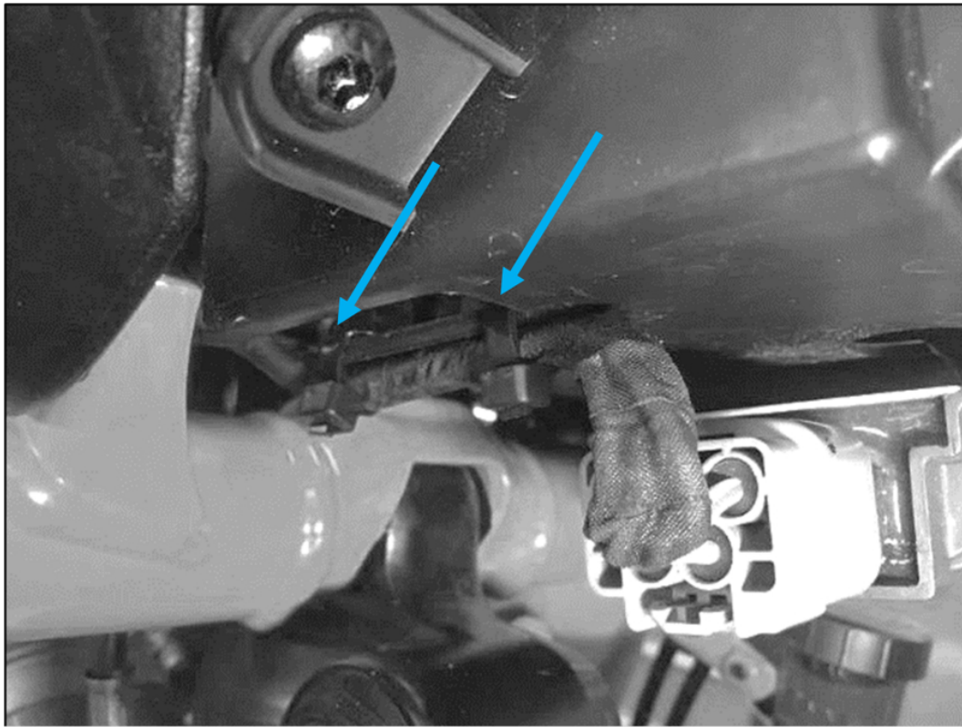
Fig. 11 - Attach the cable bundle with 2 cable ties
