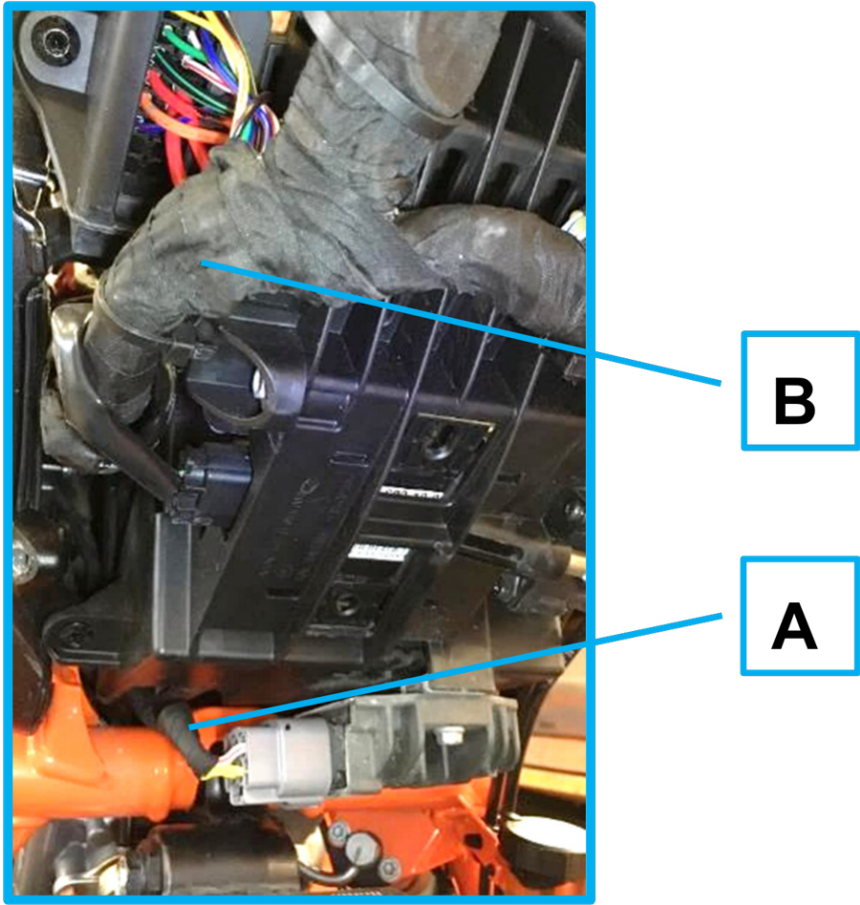
Picture 2 - Detail area A & B
