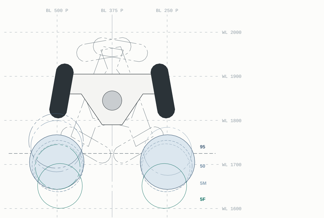
DETAIL F - YOKE SWEEP vs KNEES
