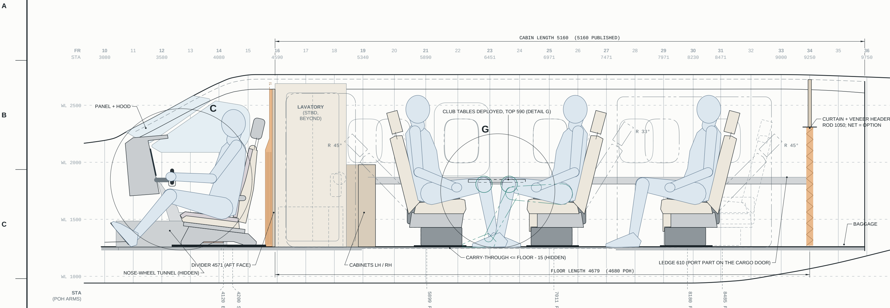
INBOARD PROFILE AT BL 375 P SEEN FROM PORT, PORT SIDEWALL REMOVED - PHANTOM R 11° RECLINE REACHED - SCALE 1:20
