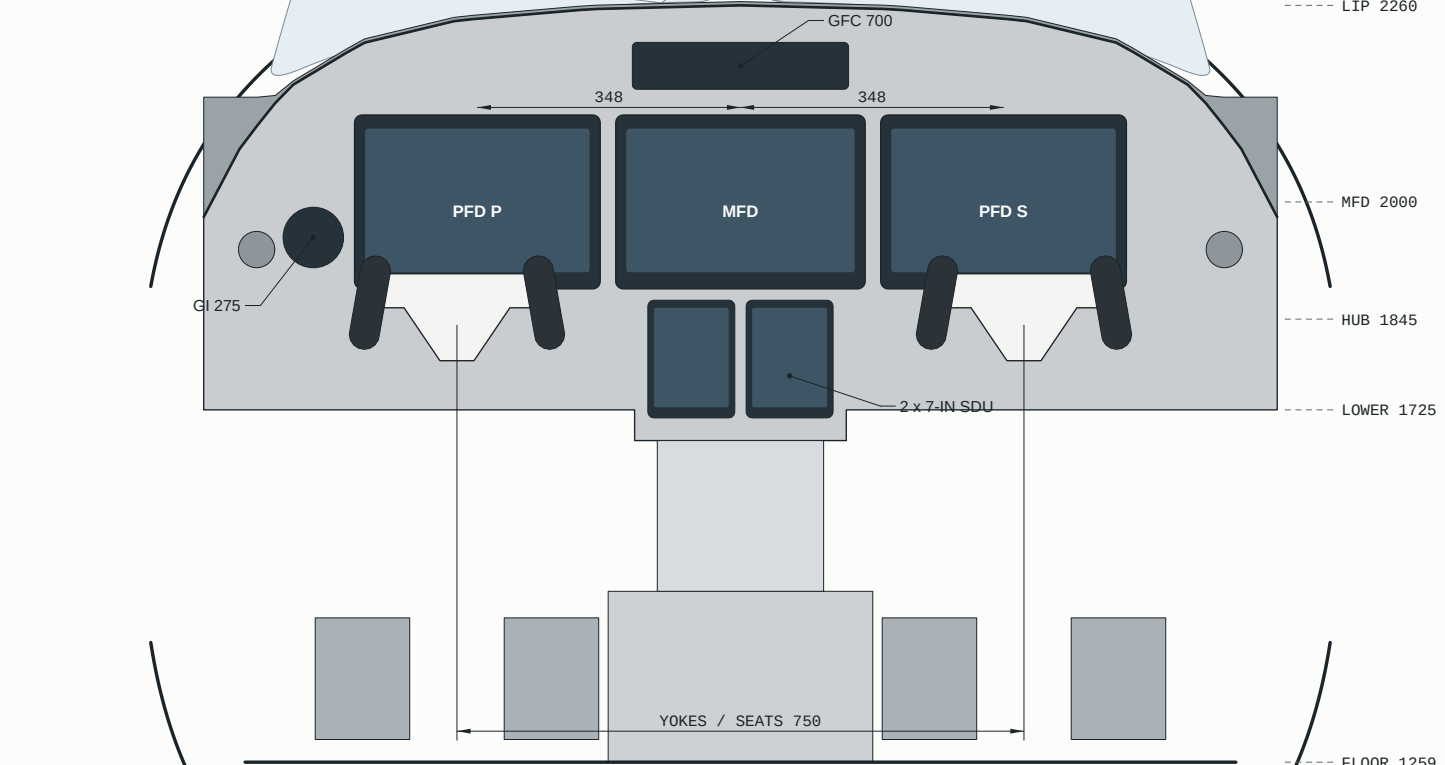
VIEW D - PANEL LOOKING FORWARD (STBD RIGHT) AT STA 3500 - SCALE 1:10
