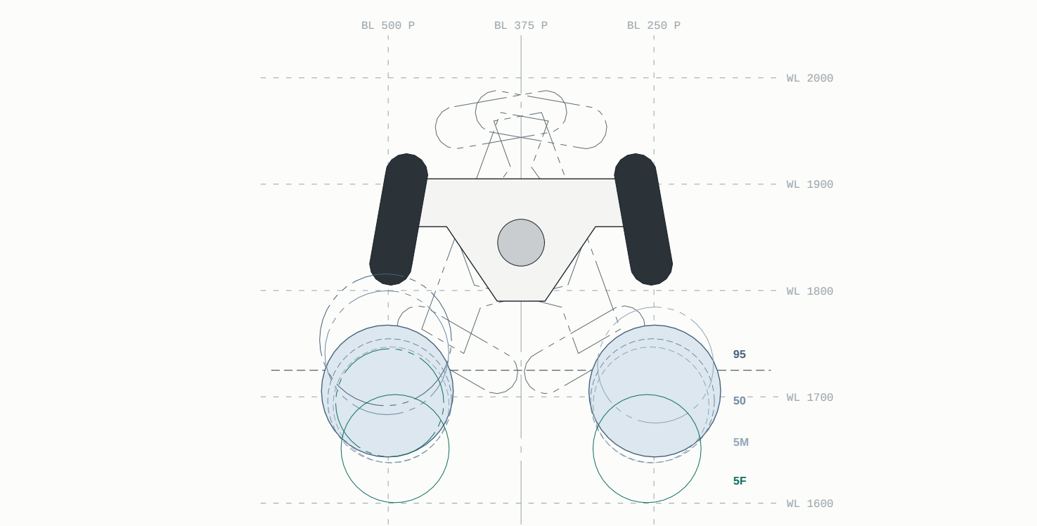
DETAIL F - YOKE SWEEP vs KNEES LEFT SEAT, LOOKING FORWARD AT THE KNEES (STA 3653) - SCALE 1:5
