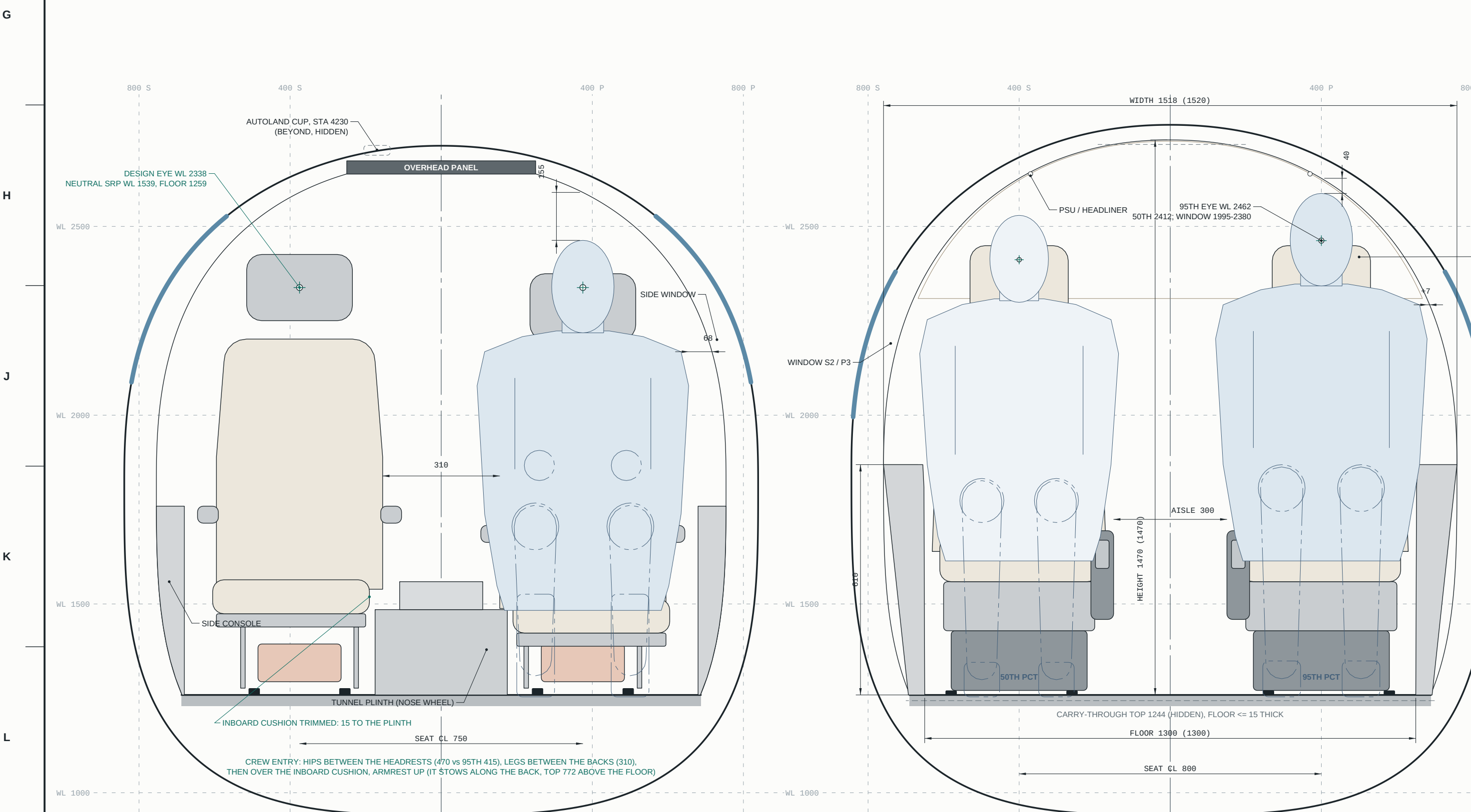
SECTION B-B STA 7011, LOOKING AFT (STBD LEFT) - SCALE 1:10 PHANTOM: KNEES, LEGS FORWARD OF THE CUT - BROWN: FR34 HEADER + ROD, BEYOND
