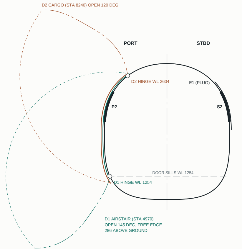
SECTION C-C - DOORS, HINGES
