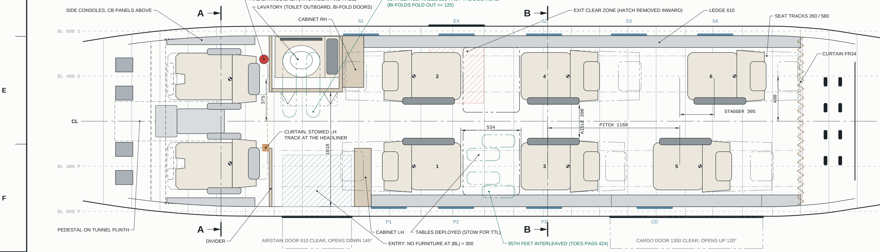
PLAN AT CUSHION HEIGHT (WL 1689)
