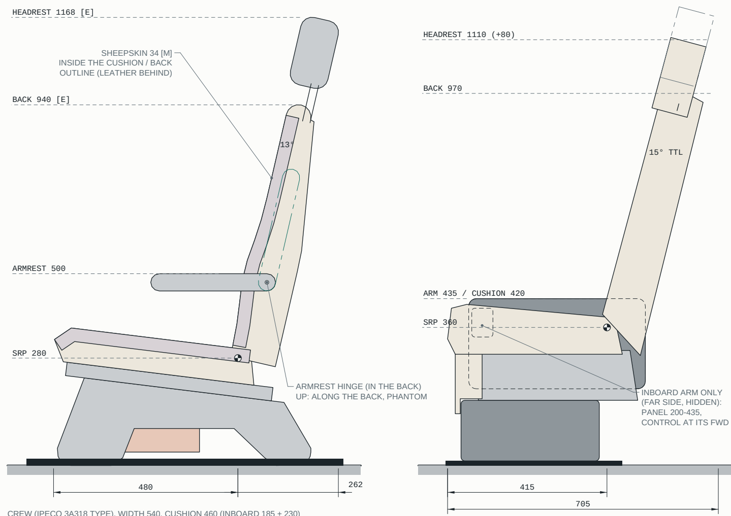
DETAIL E - SEATS
