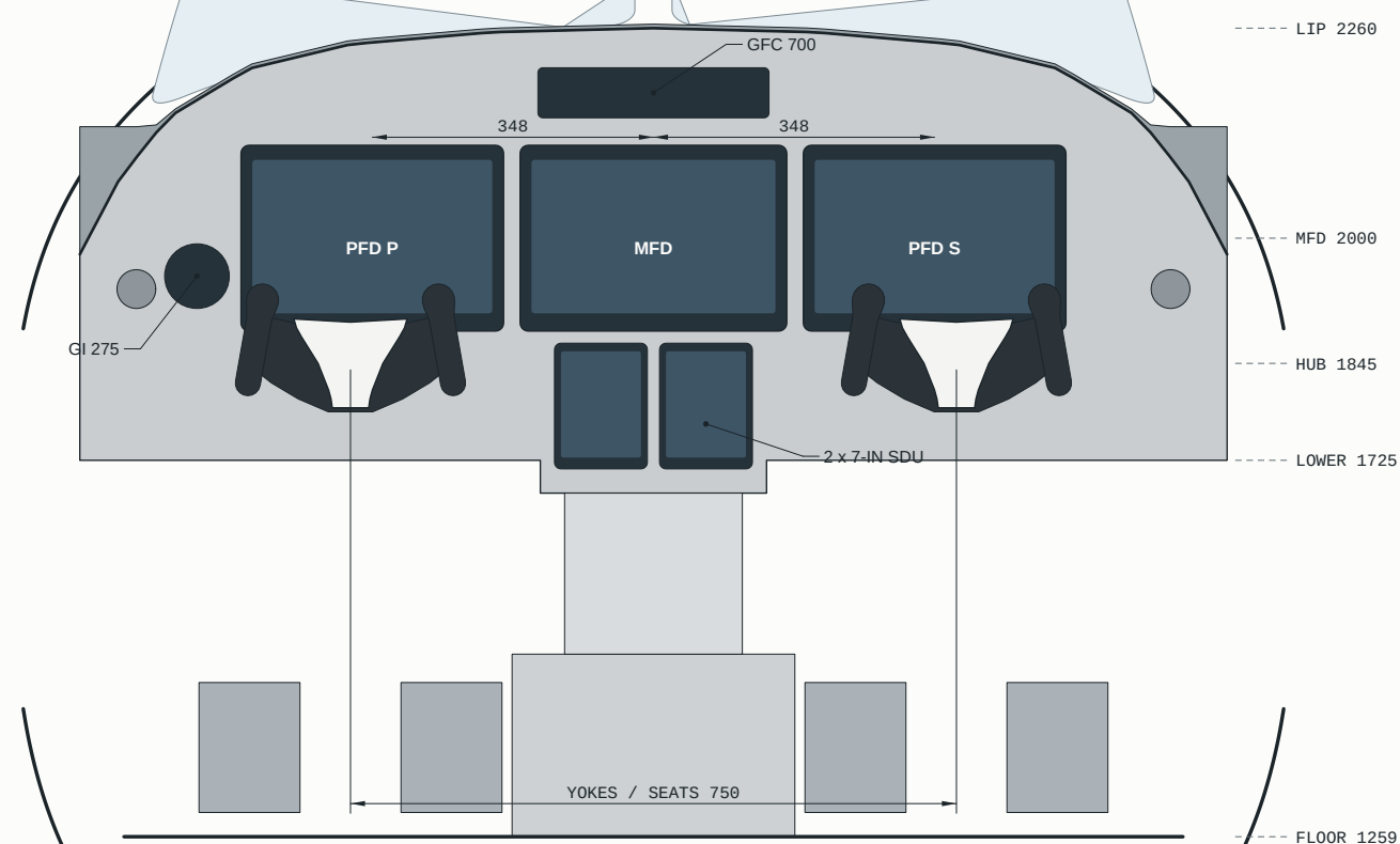
VIEW D - PANEL
