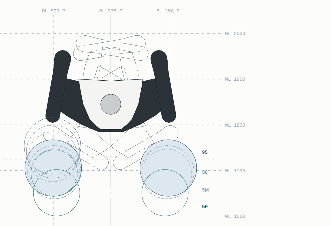
DETAIL F - YOKE SWEEP vs KNEES
