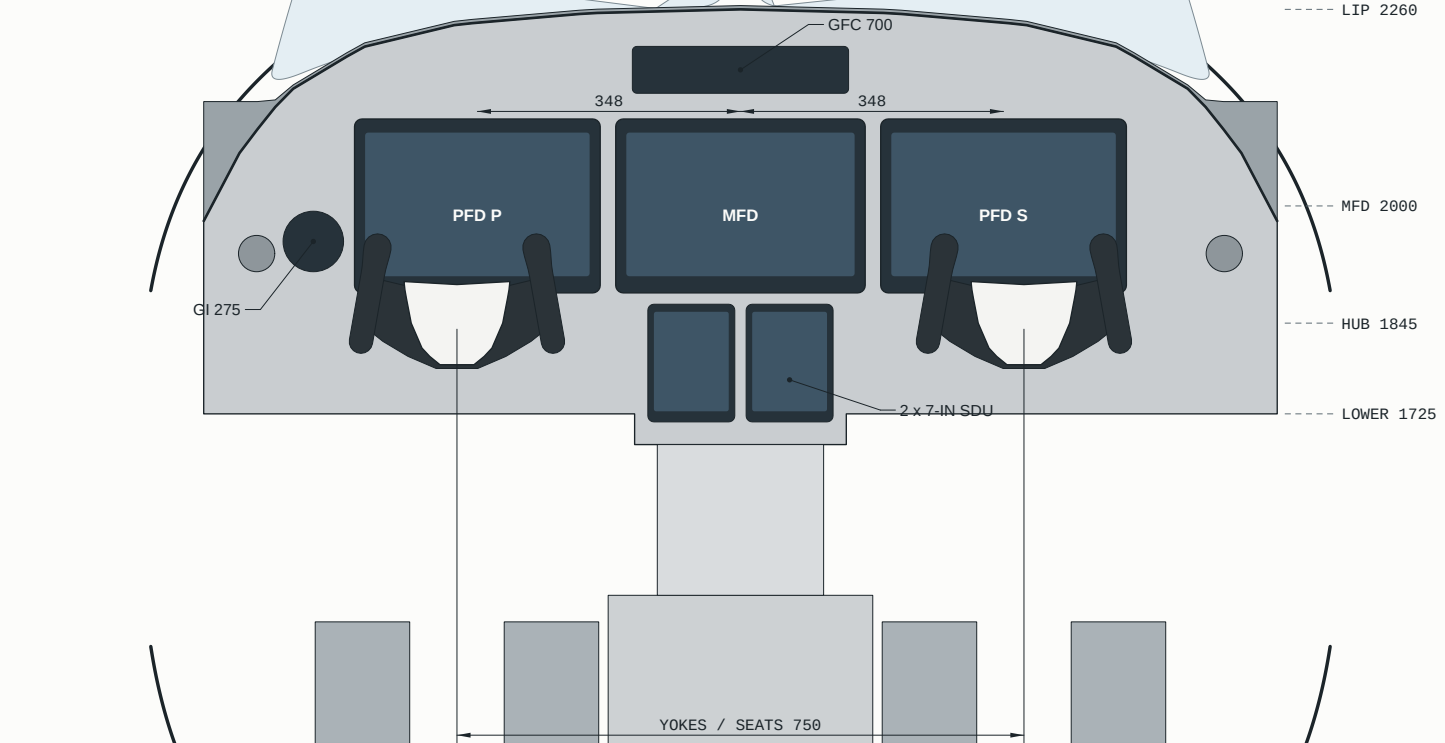
VIEW D - PANEL
