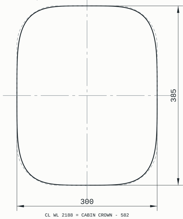
DETAIL A - CABIN WINDOW
