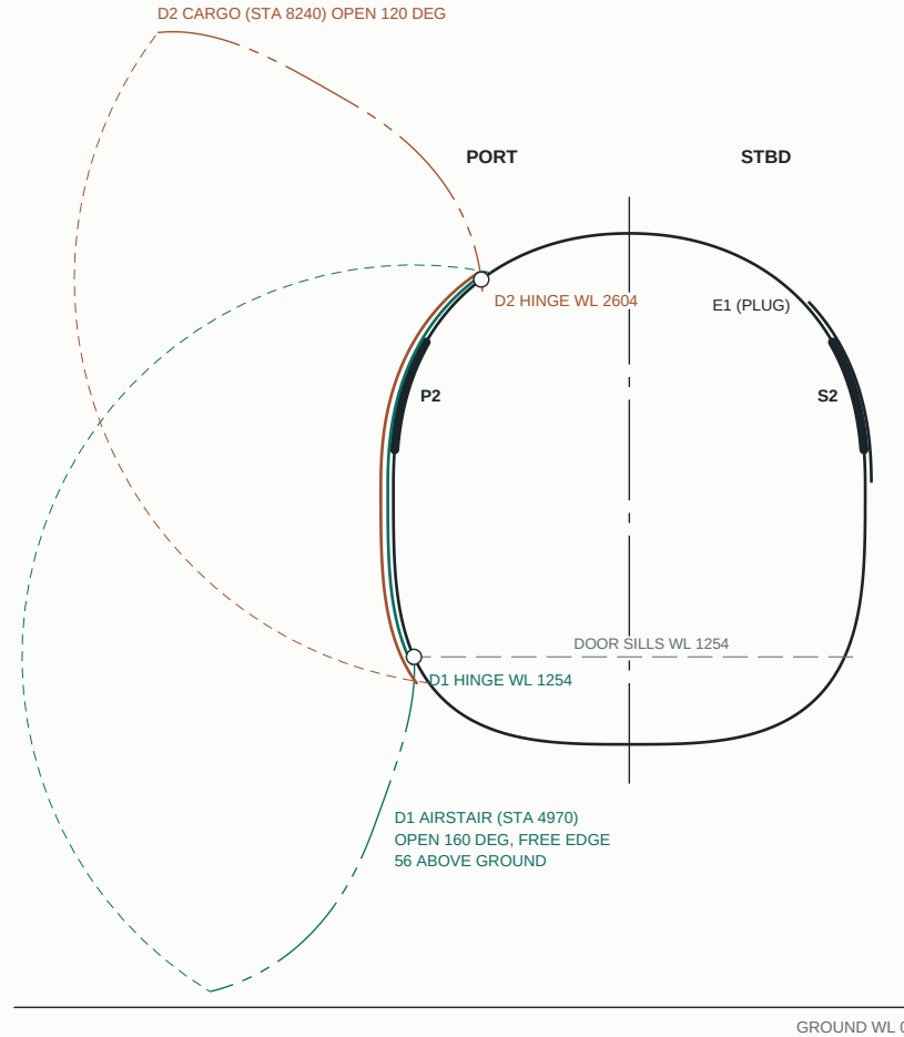
SECTION C-C - DOORS, HINGES
