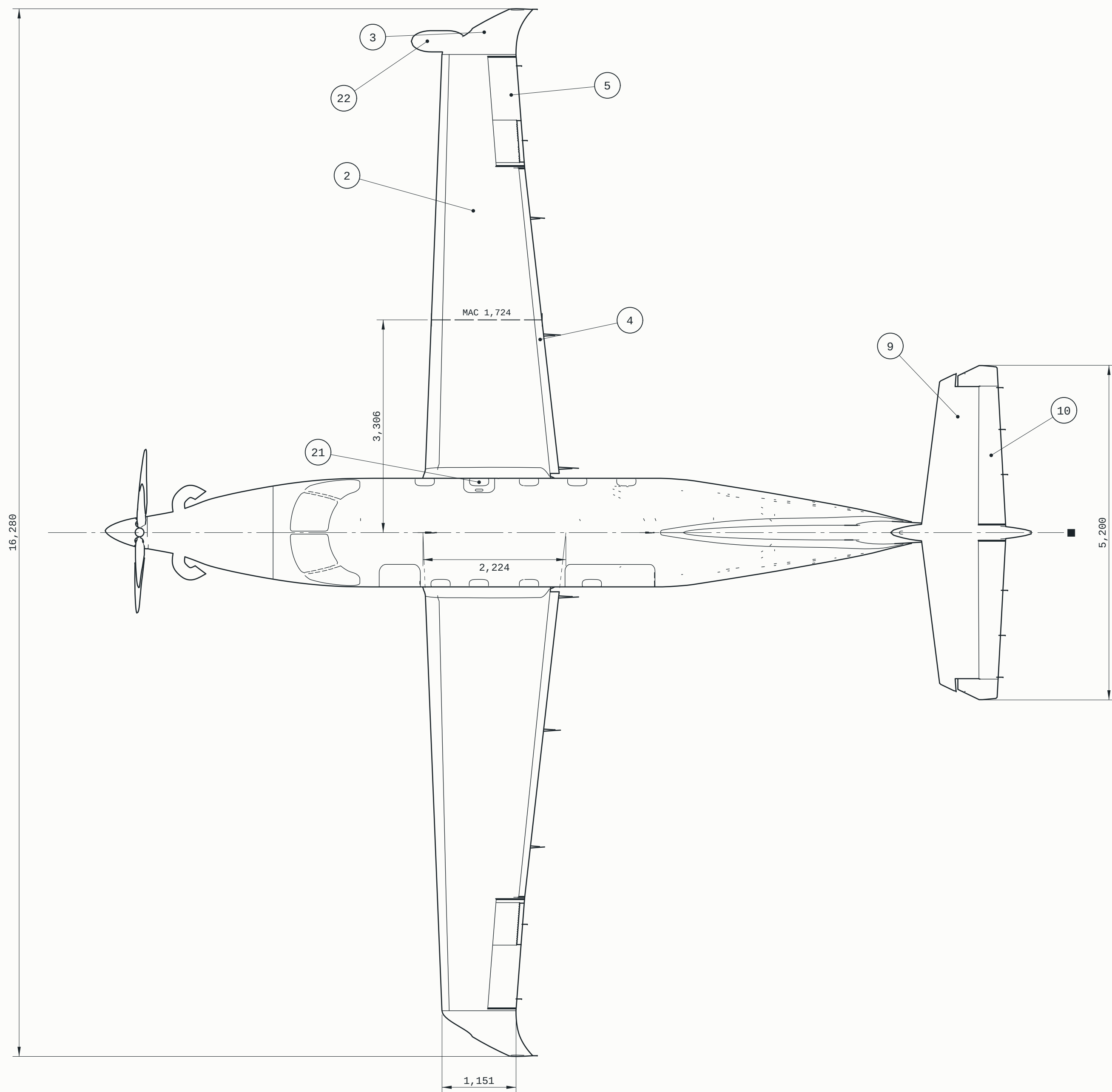
PLAN VIEW
