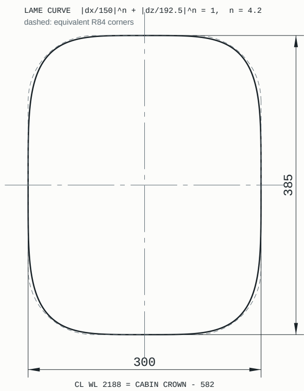
DETAIL A - CABIN WINDOW P1 (TYPICAL, ALL 9) - SCALE 1:5
