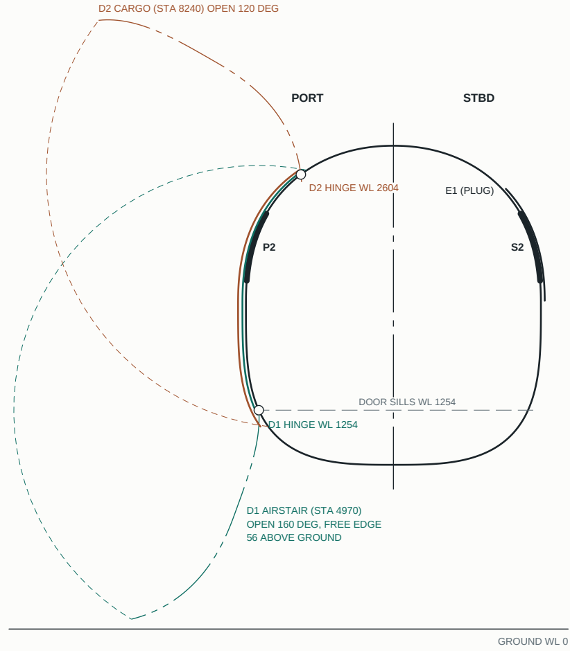
SECTION C-C - DOORS, HINGES STA 6205 LOOKING FWD - SCALE 1:30
