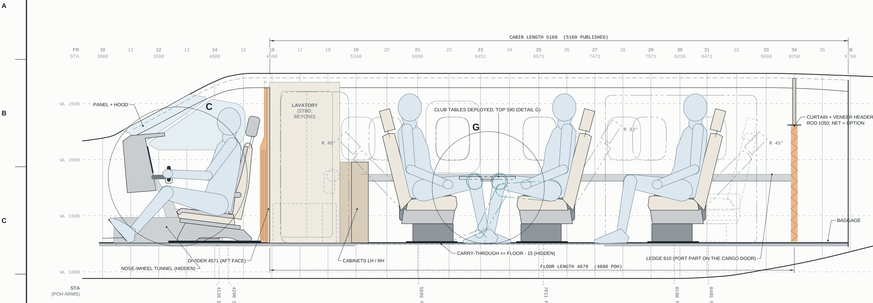
INBOARD PROFILE AT BL 375 P SEEN FROM PORT, PORT SIDEWALL REMOVED - PHANTOM R n°: RECLINE REACHED - SCALE 1:20
