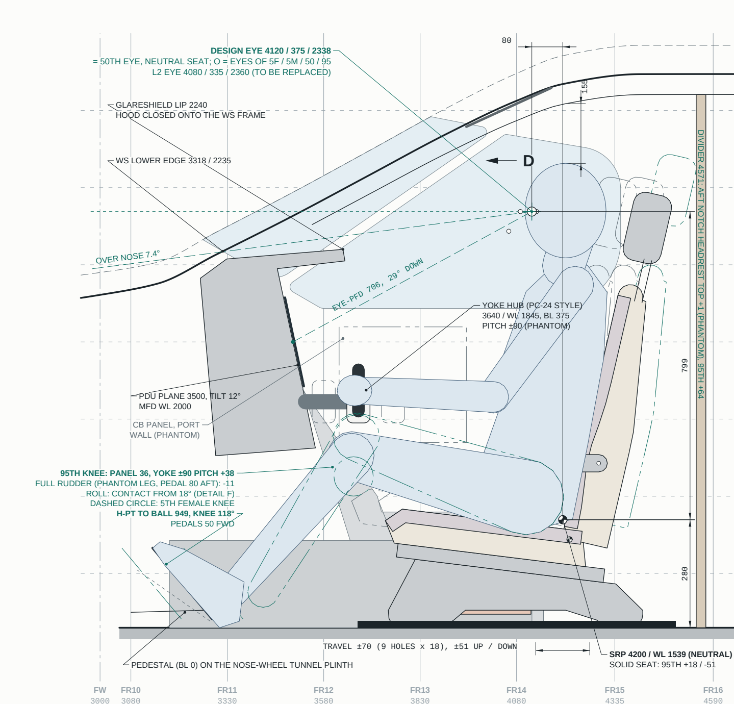
DETAIL C - CREW STATION LEFT SEAT, BL 375 P, SEEN FROM PORT - SCALE 1:10
