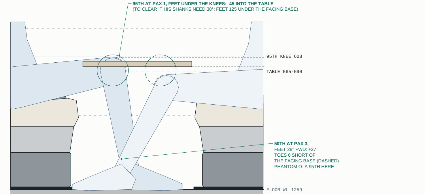
DETAIL G - CLUB TABLE vs LEGS PAX 1 (95TH) / PAX 3 (50TH), BL 400 P, SEEN FROM PORT - SCALE 1:10
