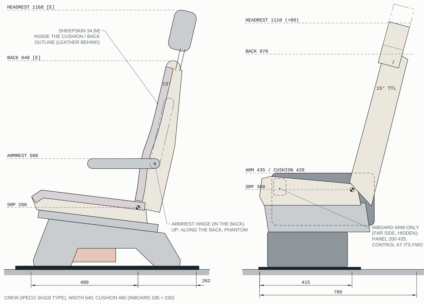
DETAIL E - SEATS CREW (NEUTRAL) / EXECUTIVE (UPRIGHT), SEEN FROM PORT - HEIGHTS ABOVE THE FLOOR - SCALE 1:10
