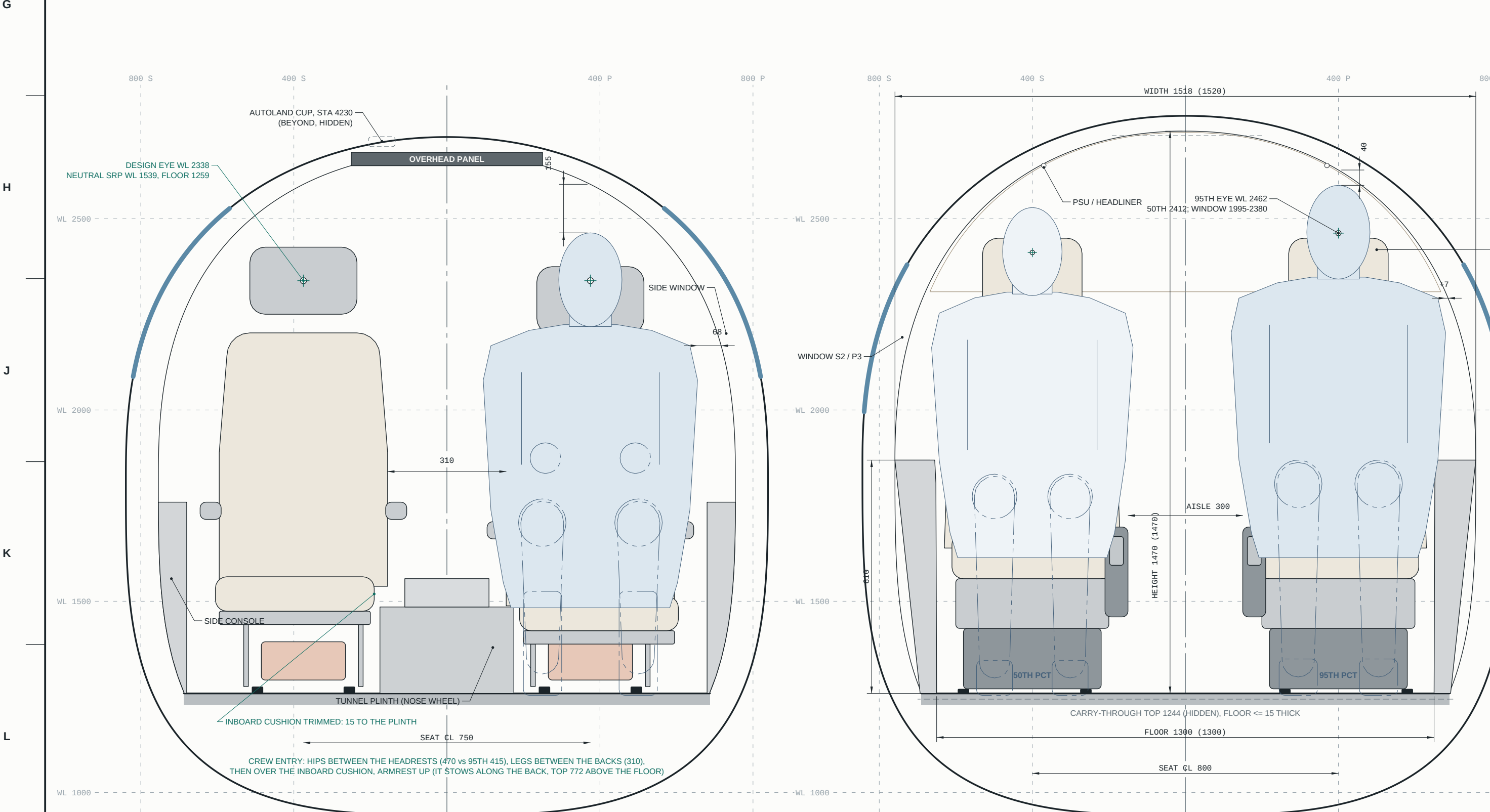
SECTION A-A STA 4120, LOOKING AFT (STBD LEFT) - SCALE 1:10 PHANTOM: KNEES, LEGS, FORWARD OF THE CUT
