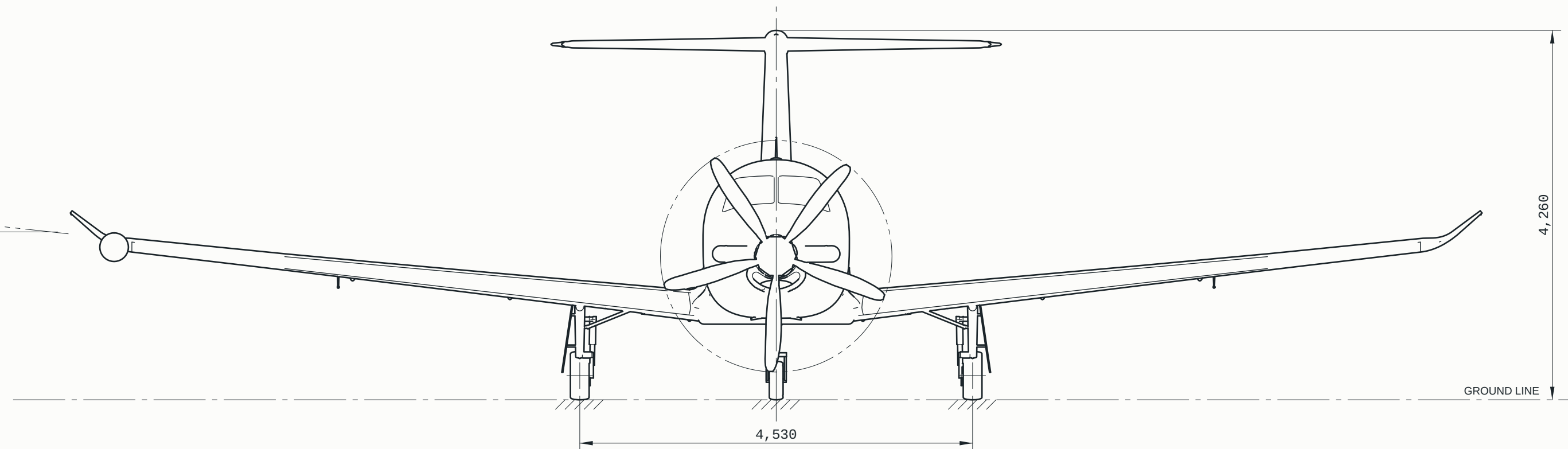
FRONT VIEW SEEN FROM AHEAD · STARBOARD ON THE LEFT
