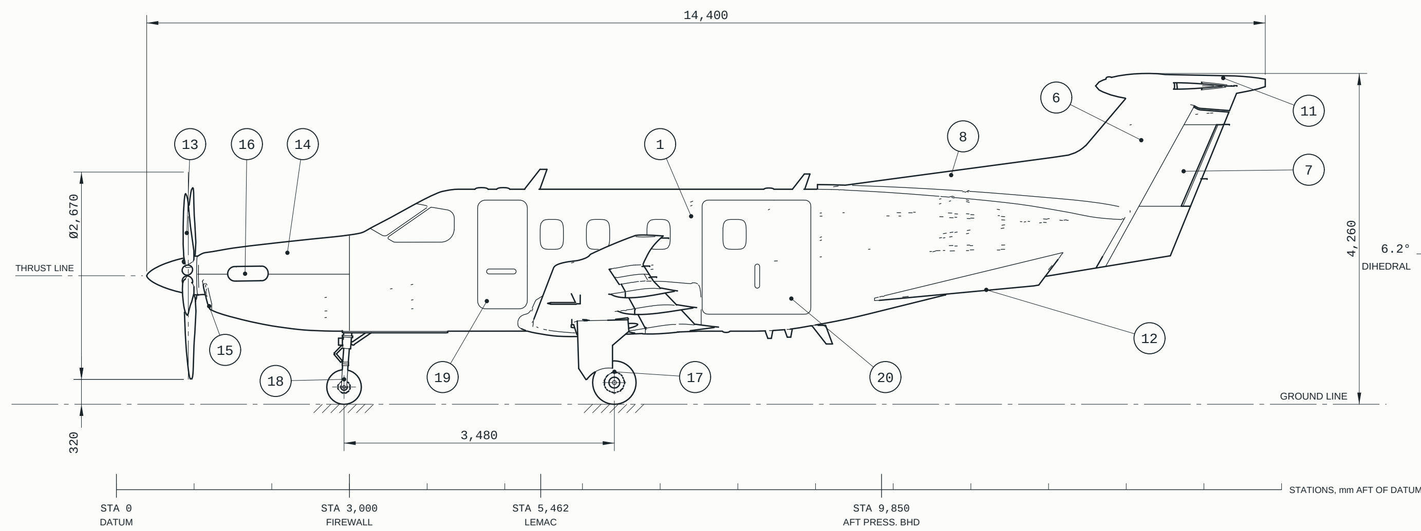
SIDE VIEW SEEN FROM PORT · NOSE LEFT
