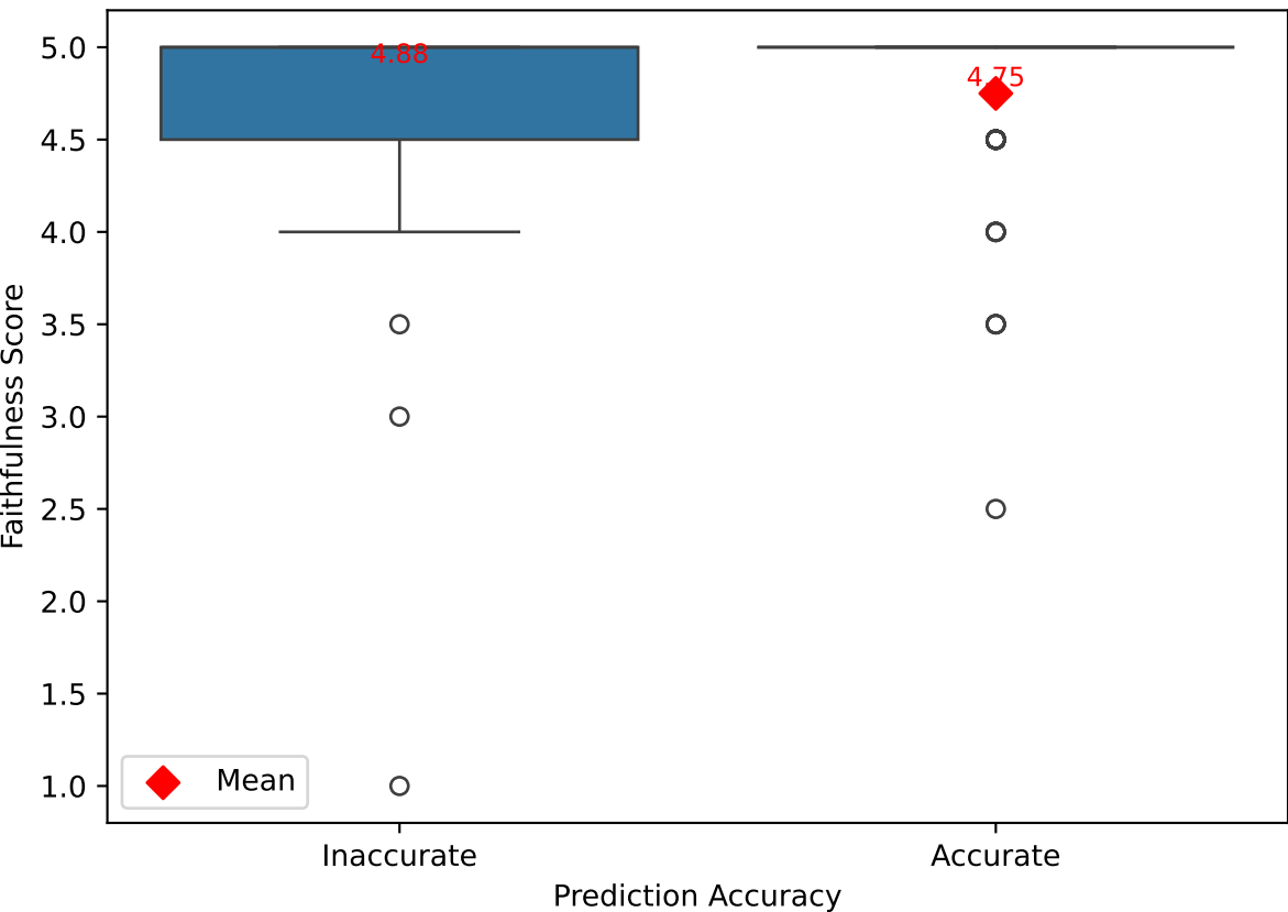
Faithfulness Score vs. Label Accuracy for G-Eval
